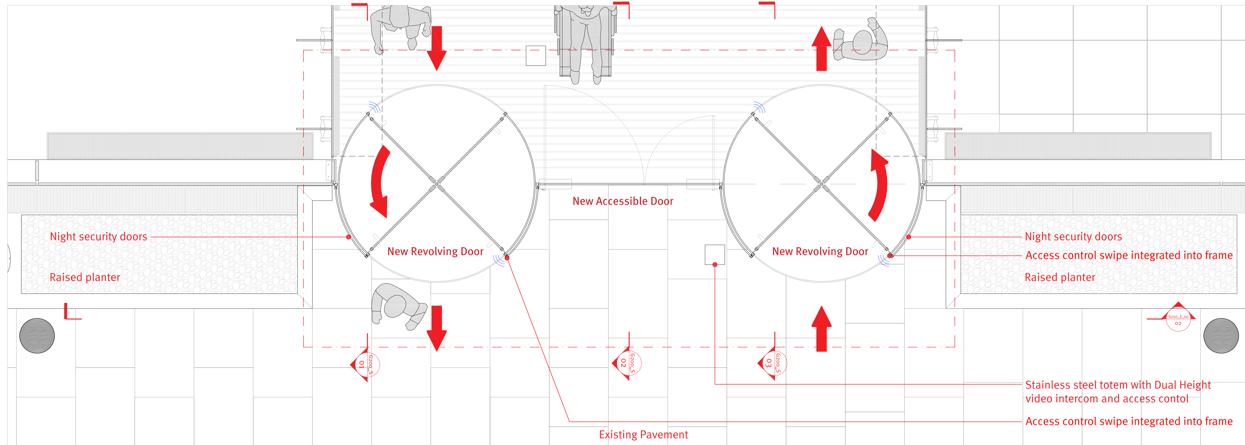
02 Details - Proposed Plan 1:20 @ A1
