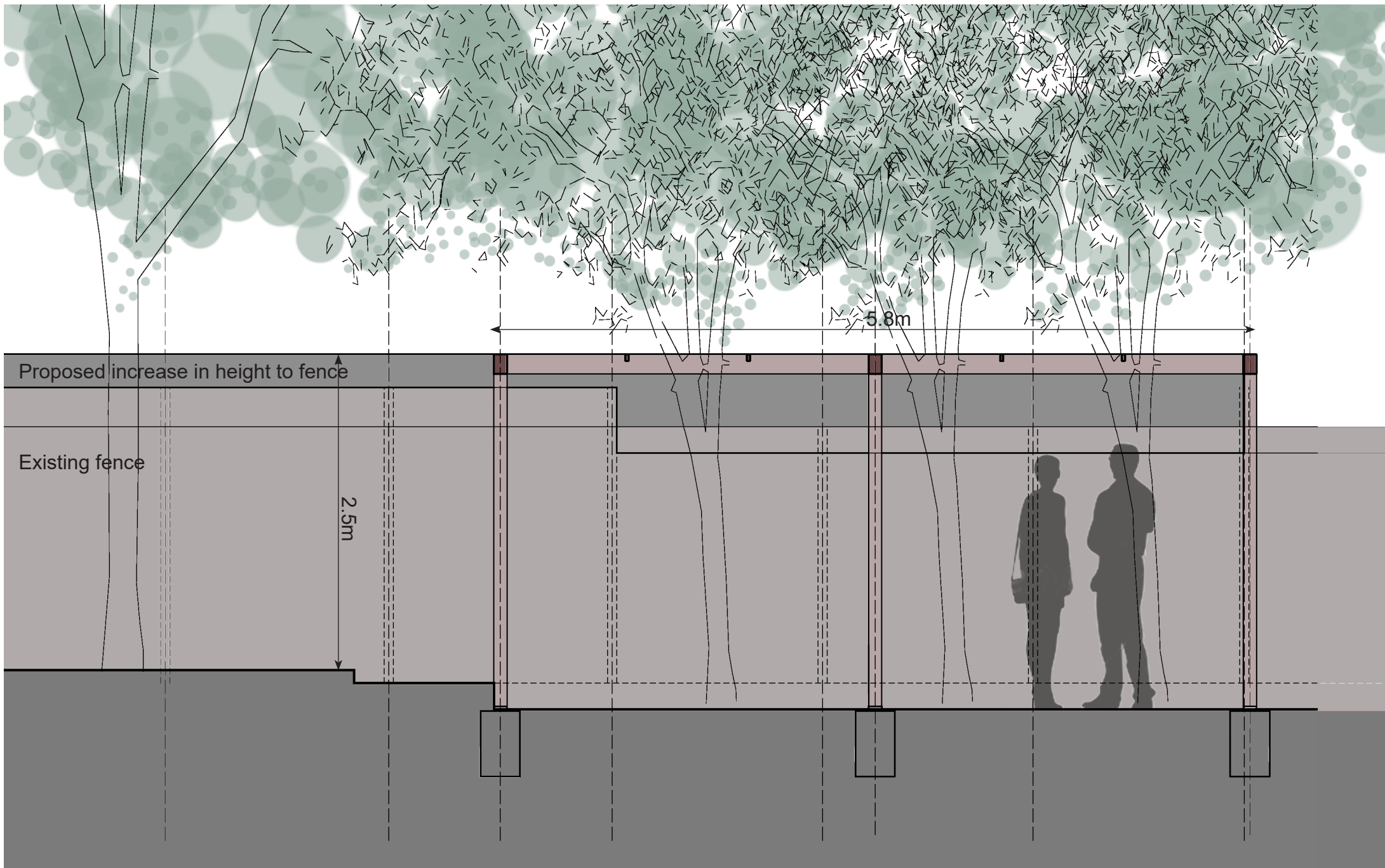
Section looking towards 42 - 51 Clevedon Mansions Drawing number : P_03 Scale 1: 25 @ A4
