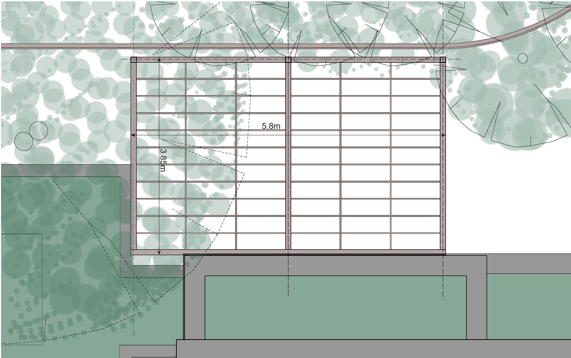
Proposed plan of pergola Drawing number : P_02 Scale 1: 35 @ A4
