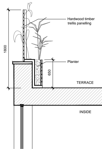
Section through screening
