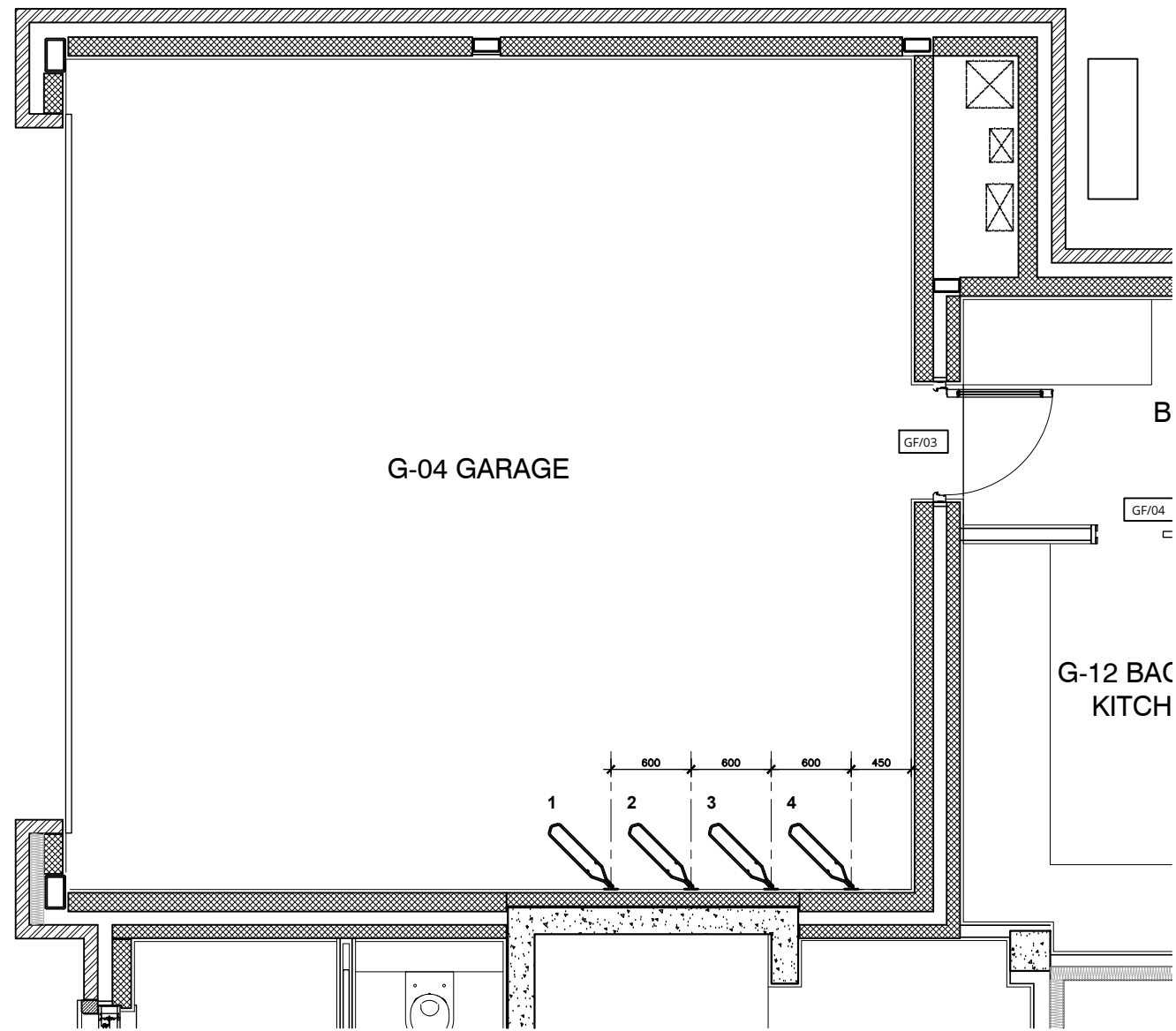
Partial Ground Floor Plan SCALE 1:50
