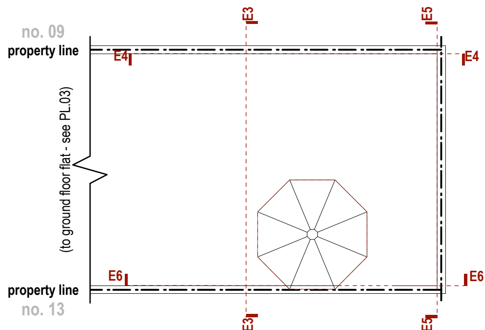
Existing Garden Shed/Outhouse Roof Plan
