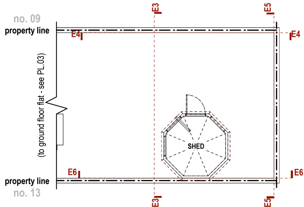
Existing Garden Shed/Outhouse Plan
