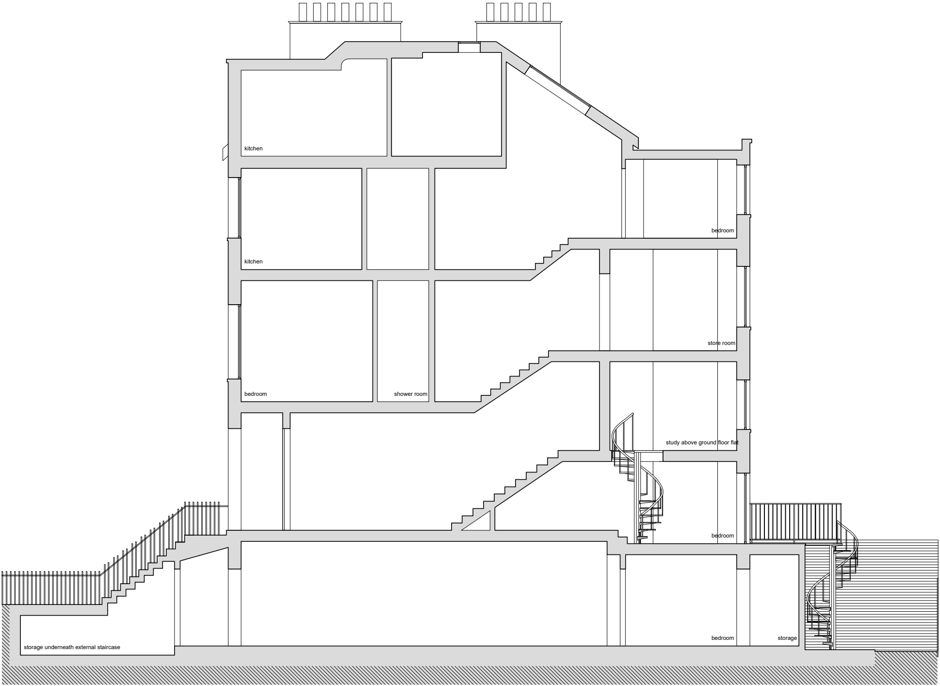
Section EE Existing
