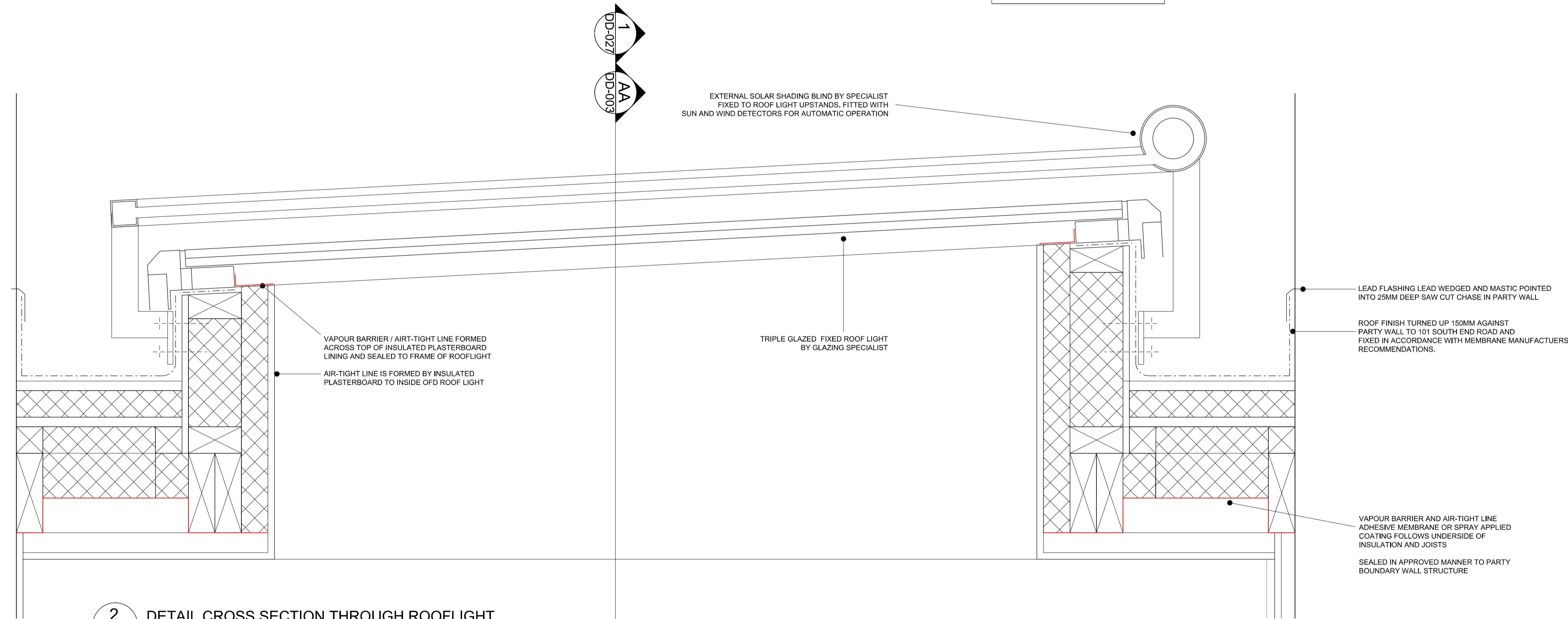
2 DETAIL CROSS SECTION THROUGH ROOFLIGHT WITH ROOF ABUTMENT TO PARTY WALL DD-027
