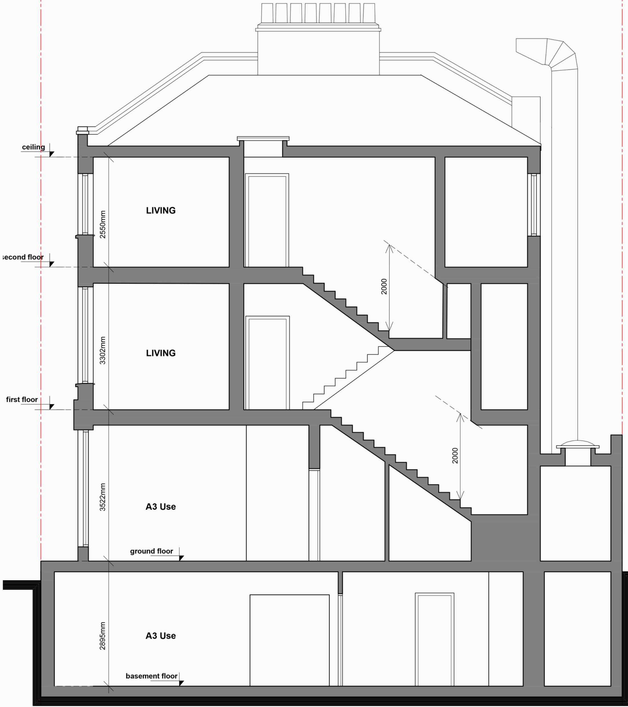
APPROVED LONGITUDINAL SECTION A - A' SCALE 1/50 at A3
