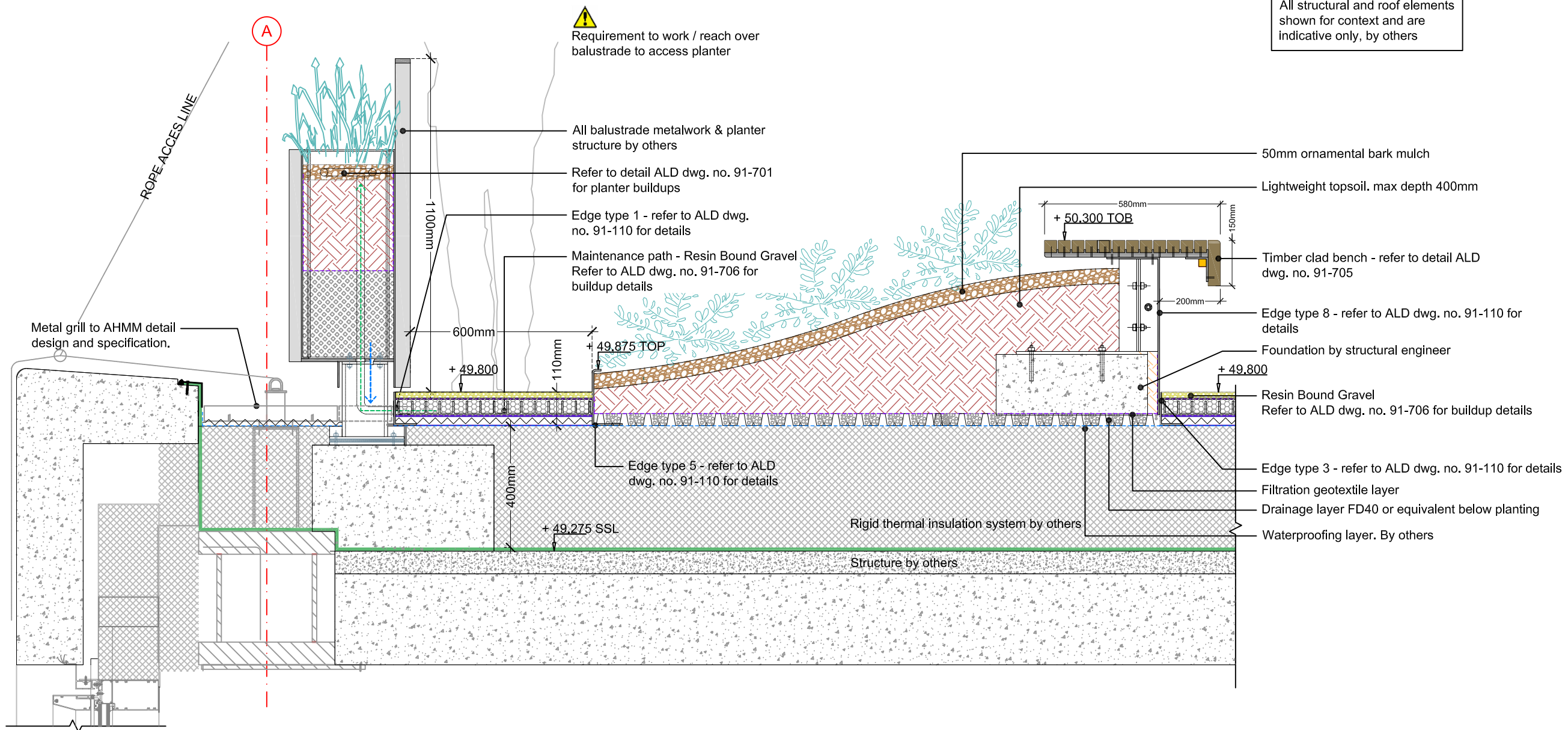
022 DETAIL THROUGH TERRACE BALUSTRADE PLANTER AT LEG LOCATIONS, MAINTENANCE PATH , PLANTING BED & BENCH SCALE: 1:15 @ A3
