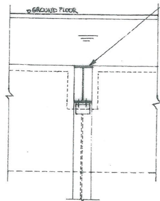
DETAIL A-A (1:10)
