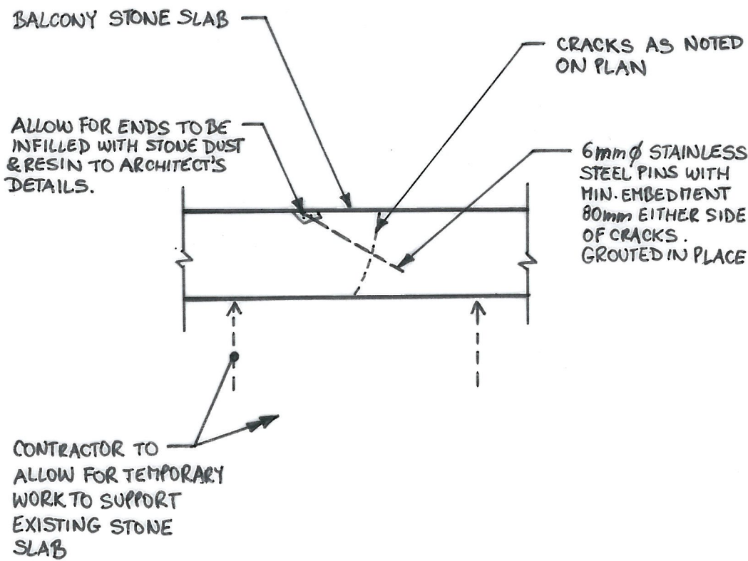
DETAIL 04 (1:5)
