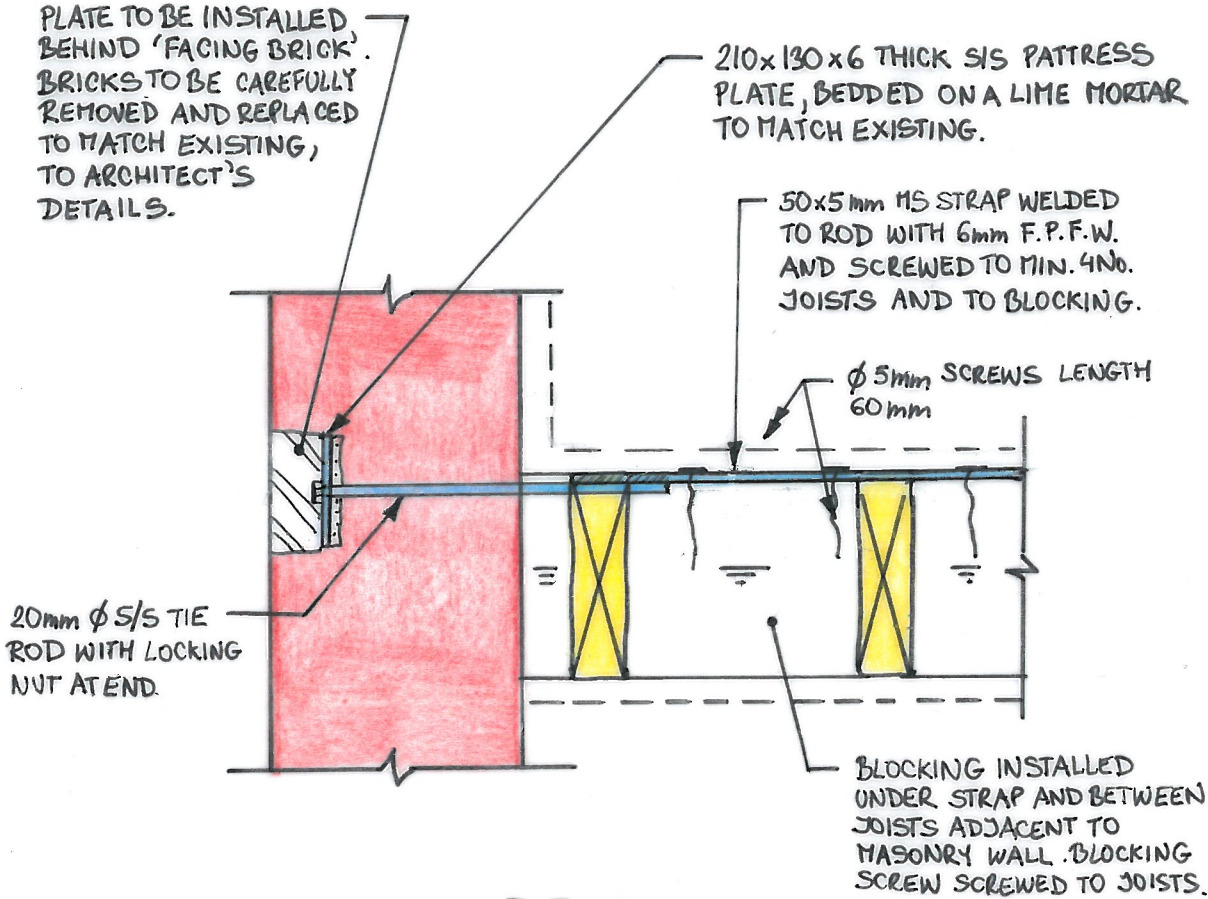
DETAIL 02 (1:10)
