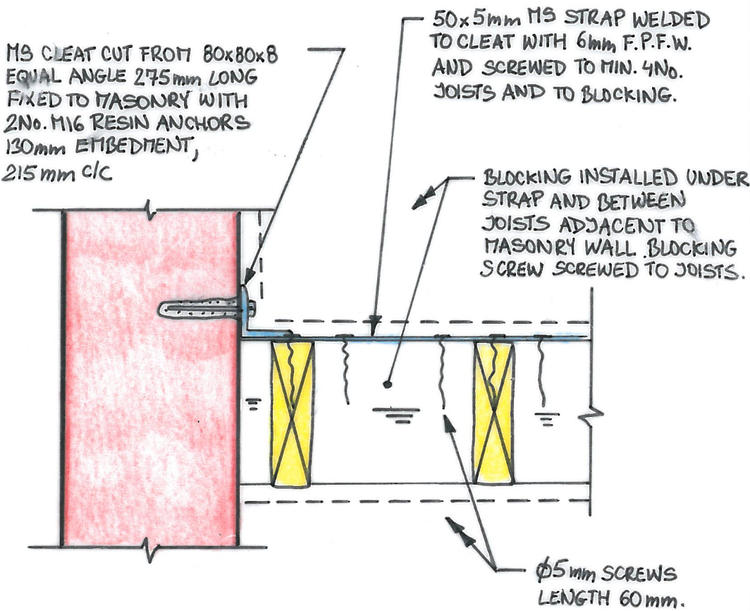
DETAIL 01 (1:10)
