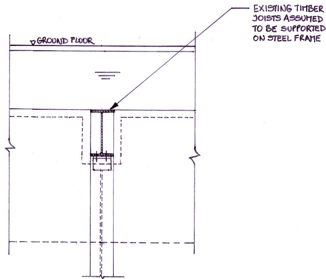
DETAIL A-A (1:10)
