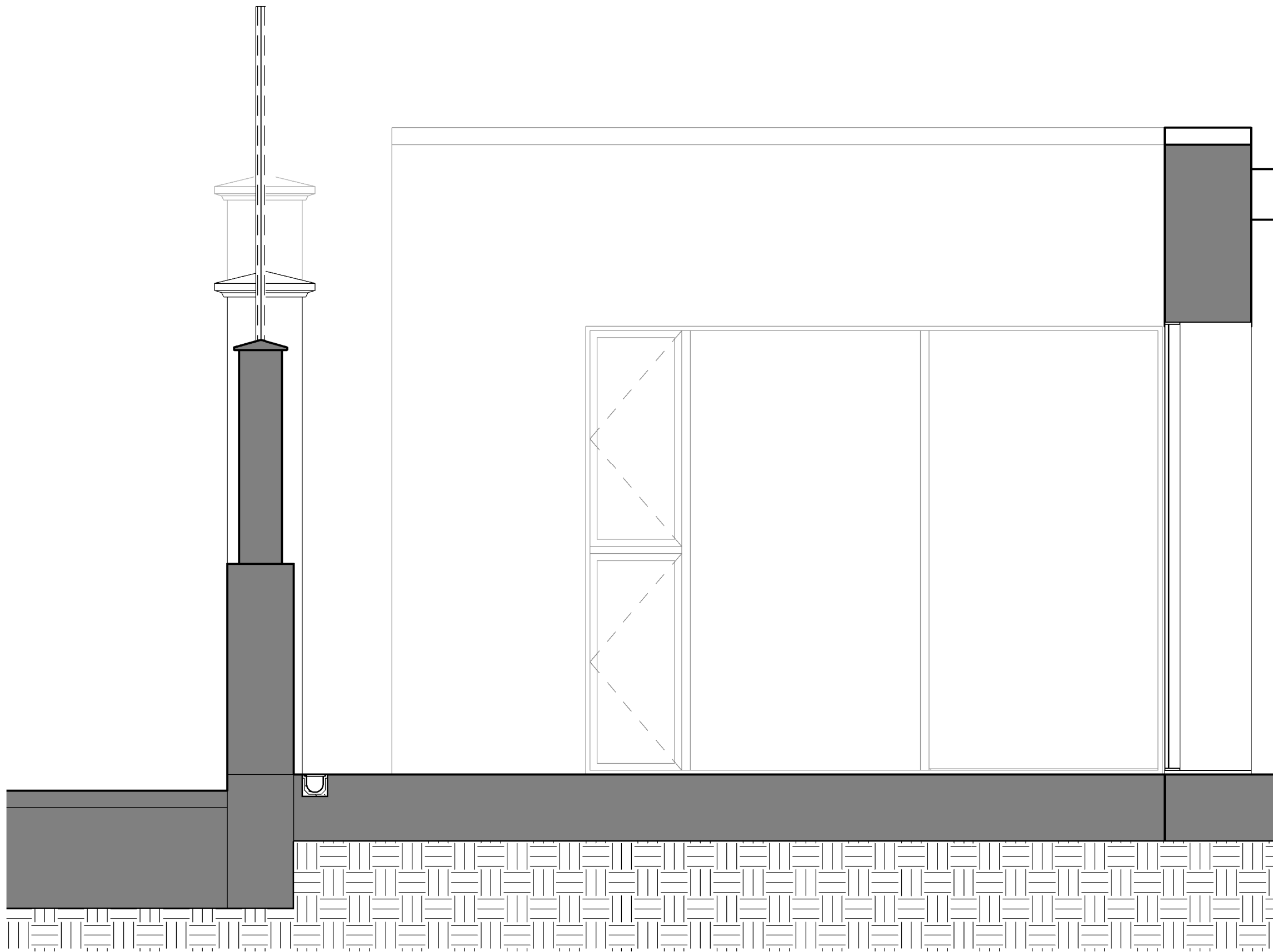
1 Cross Section_Existing 1 : 25
