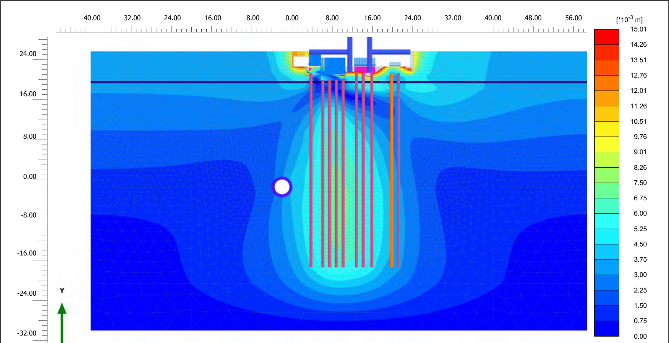
Total displacements |u| (Time 375.0 day)
