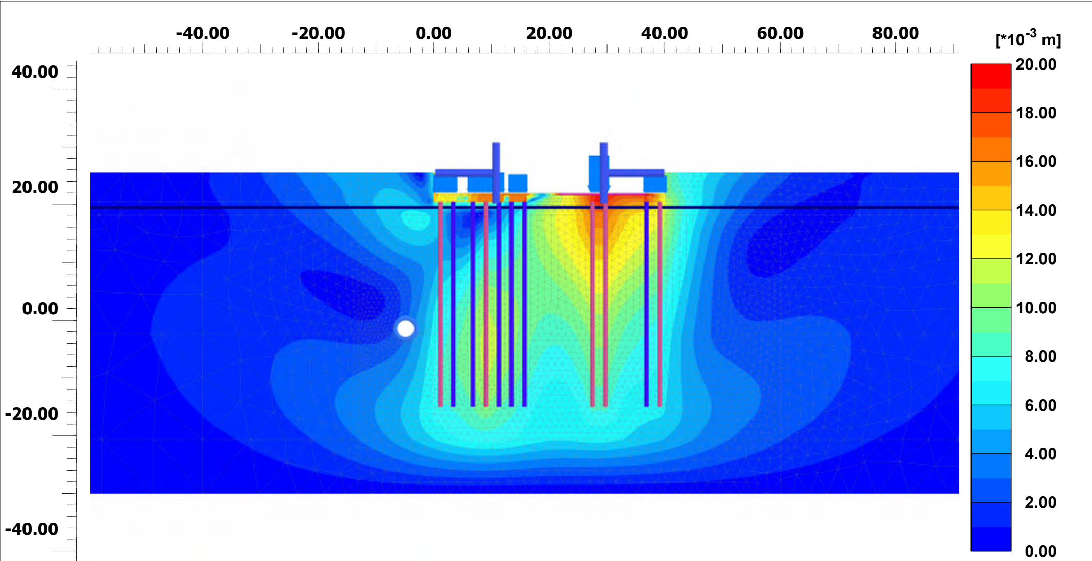
Total displacements |u|
