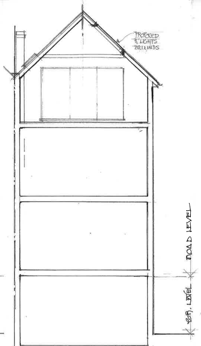
SECTION AA (PROPOSED)
