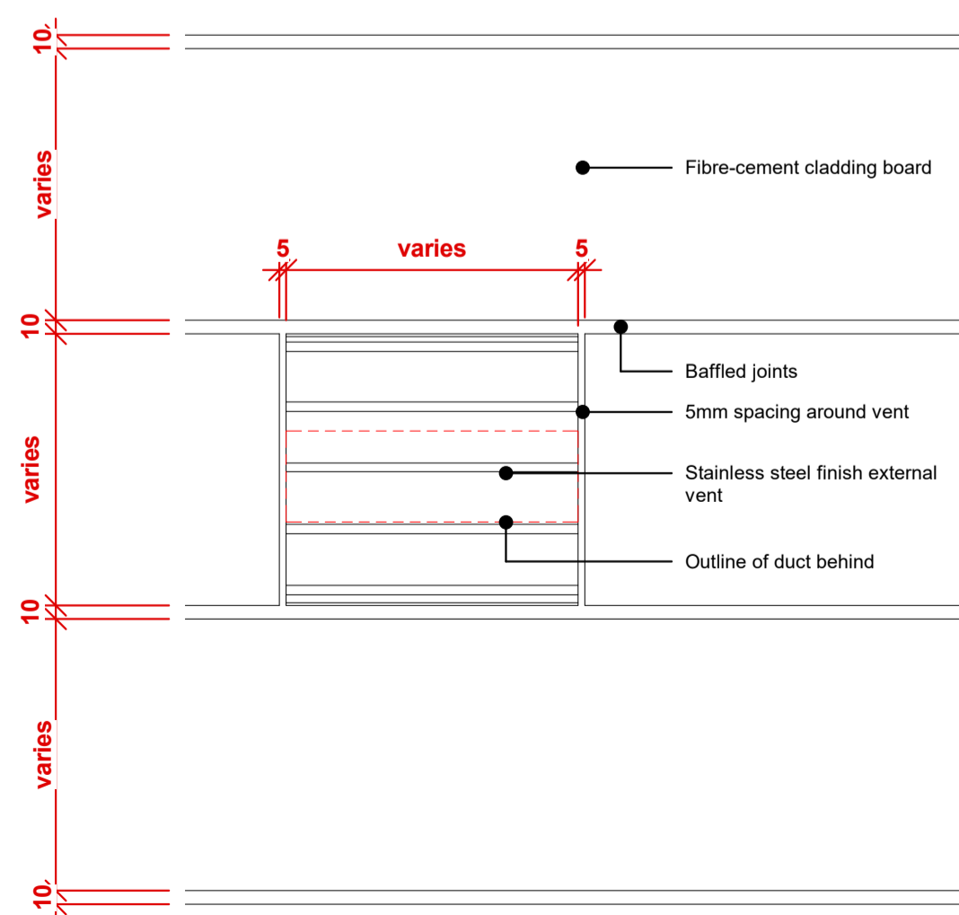
2 Typical Vent Fibre Cement Cladding Elevation Detail Scale 1 : 5
