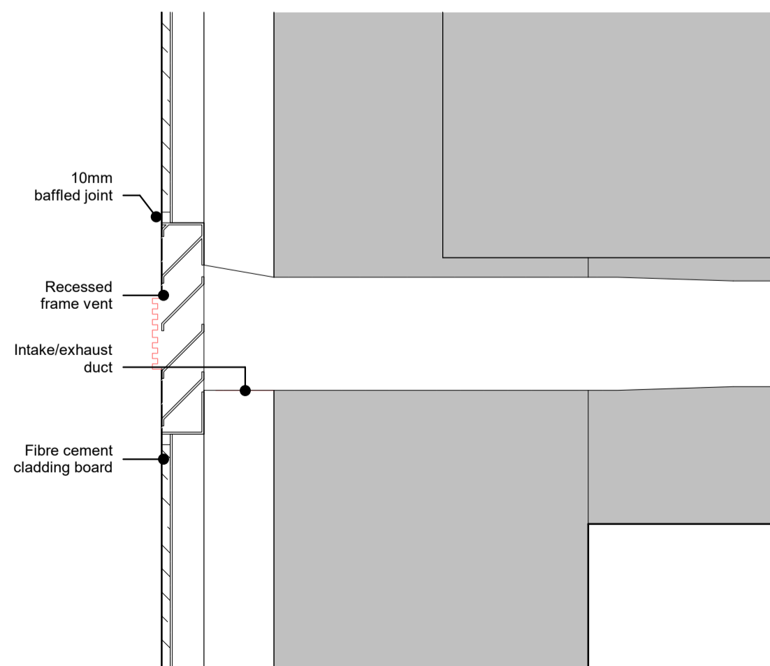
3 Typical Vent Fibre Cement Cladding Section Detail Scale 1 : 5
