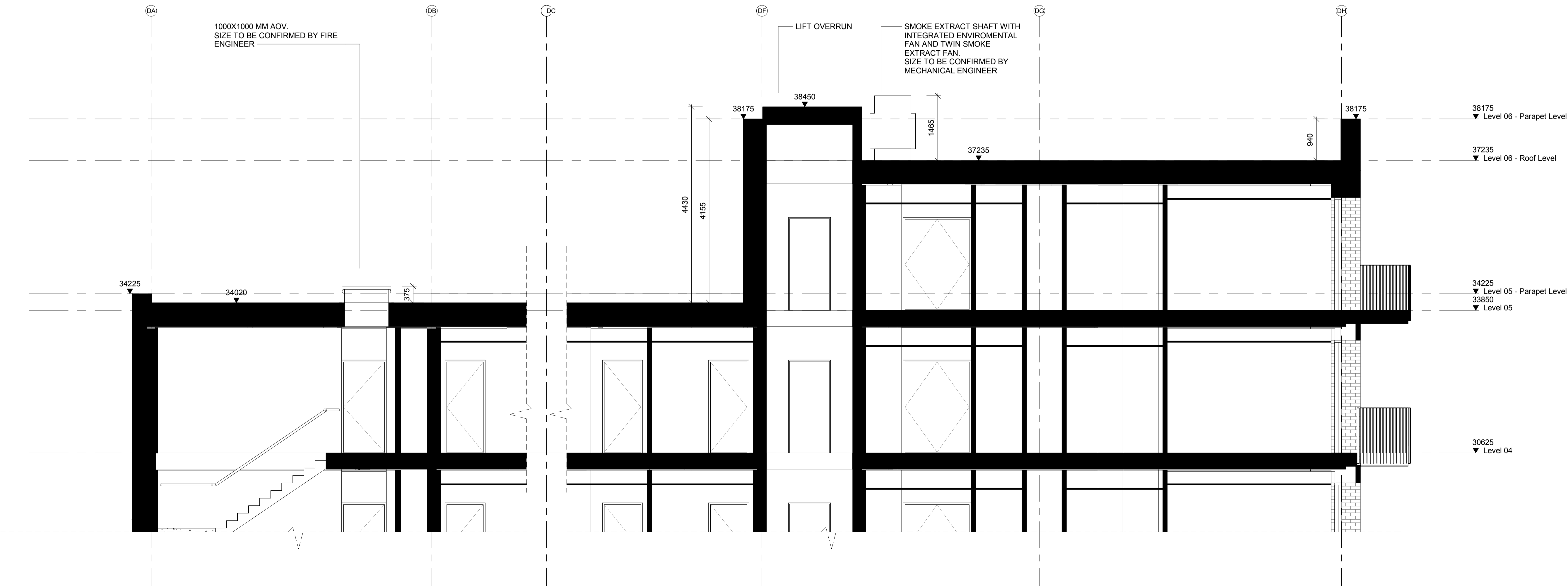
Roof Section - Block D - Generic heights
