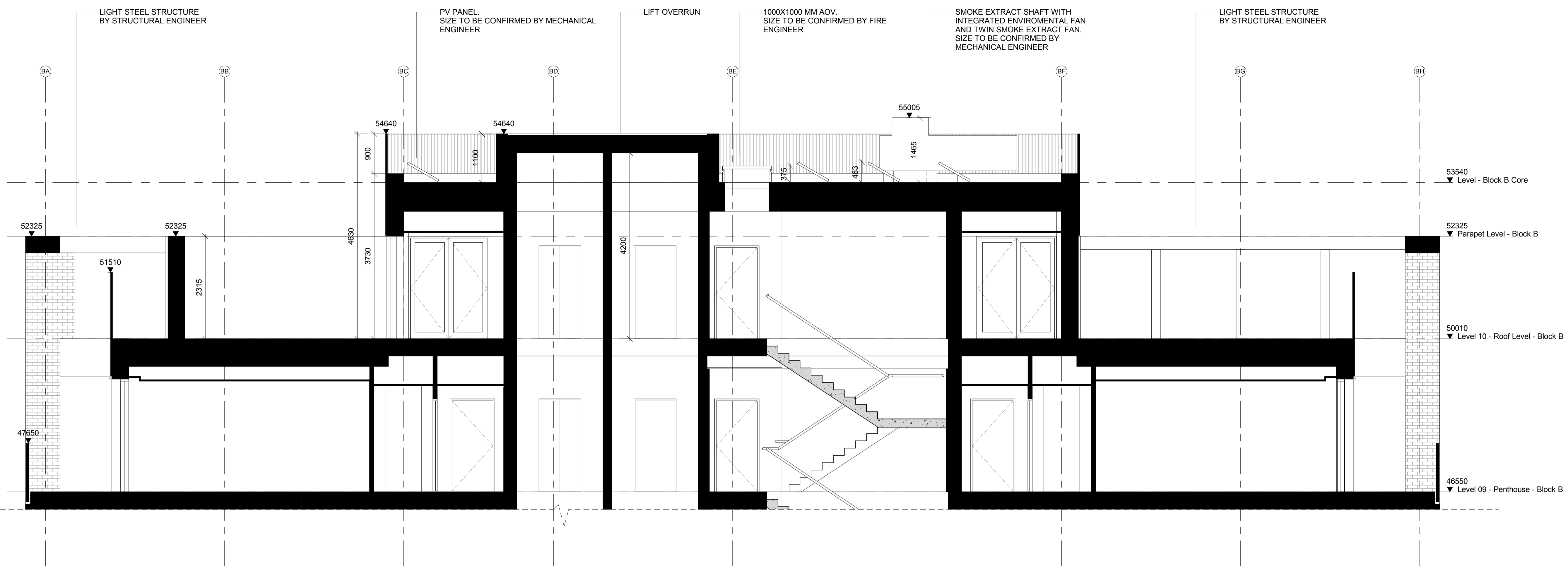
Roof Section - Block B - Generic heights
