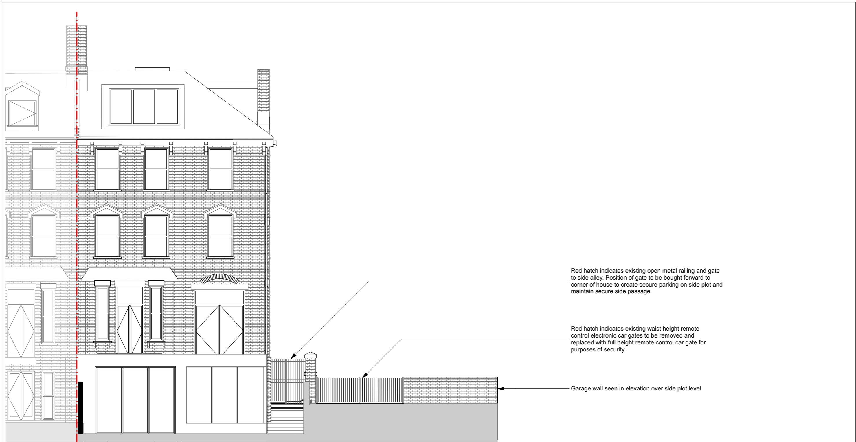
Rear Elevation
