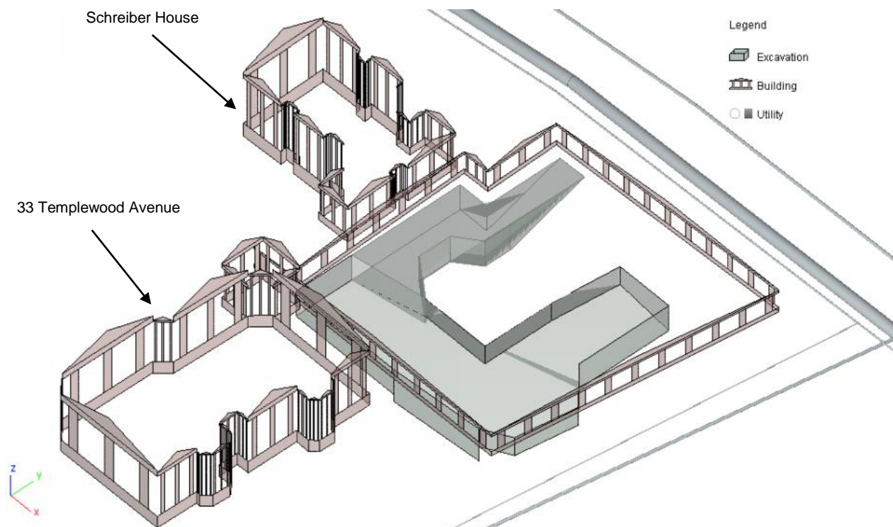
Figure 16.6: Indicative plot of the three-dimensional analytical model produced using the Oasys software suite (soil and Thames Water assets removed for clarity of presentation). Simplified excavation geometry shown in green.
