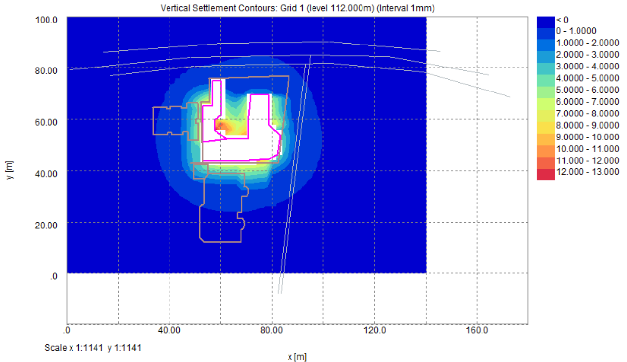
Figure 16.18: Vertical Movement – Method 2 – CIRIA curves + Long-term loading
