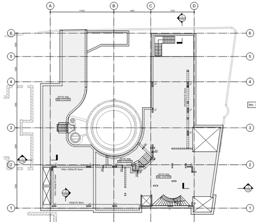
(a) Proposed scheme ground level plan
