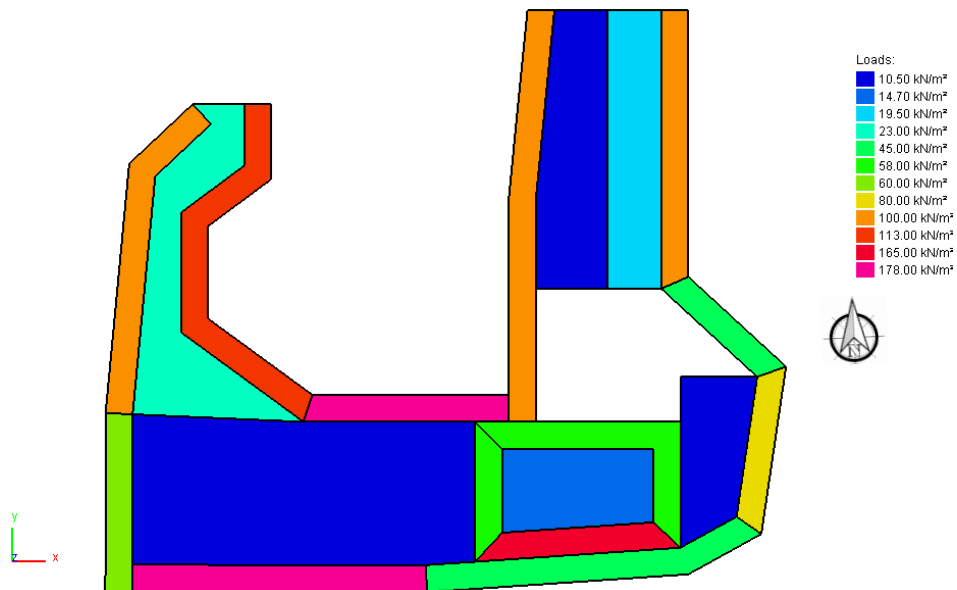
Figure 16.7: Idealised long-term loading regime modelled in Pdisp
