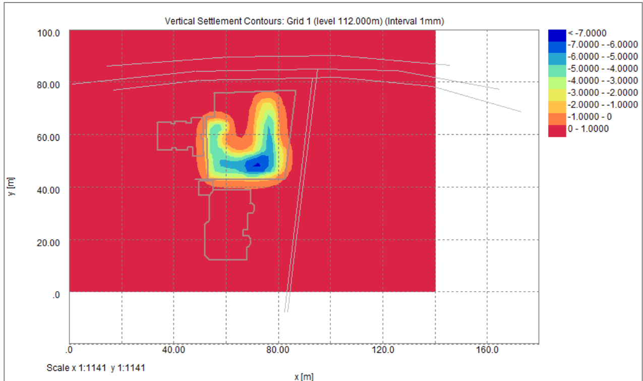
Figure 16.11: Vertical Movement – Method 1 after Excavation
