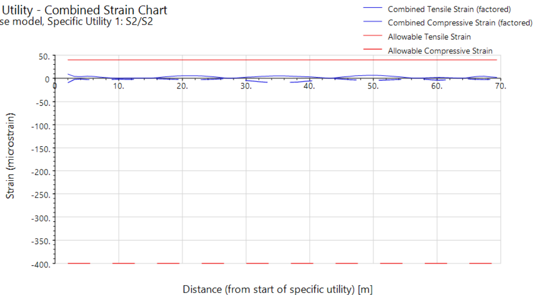
Figure 16.17: Combined strain profile of Sewer S2 – Method 2 CIRIA Excavation and Installation - based on smoothed deflection profile
