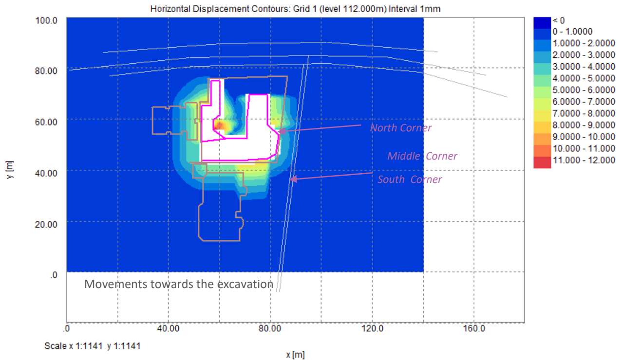
Figure 16.14: Horizontal Movement – Method 2 CIRIA Excavation and Installation
