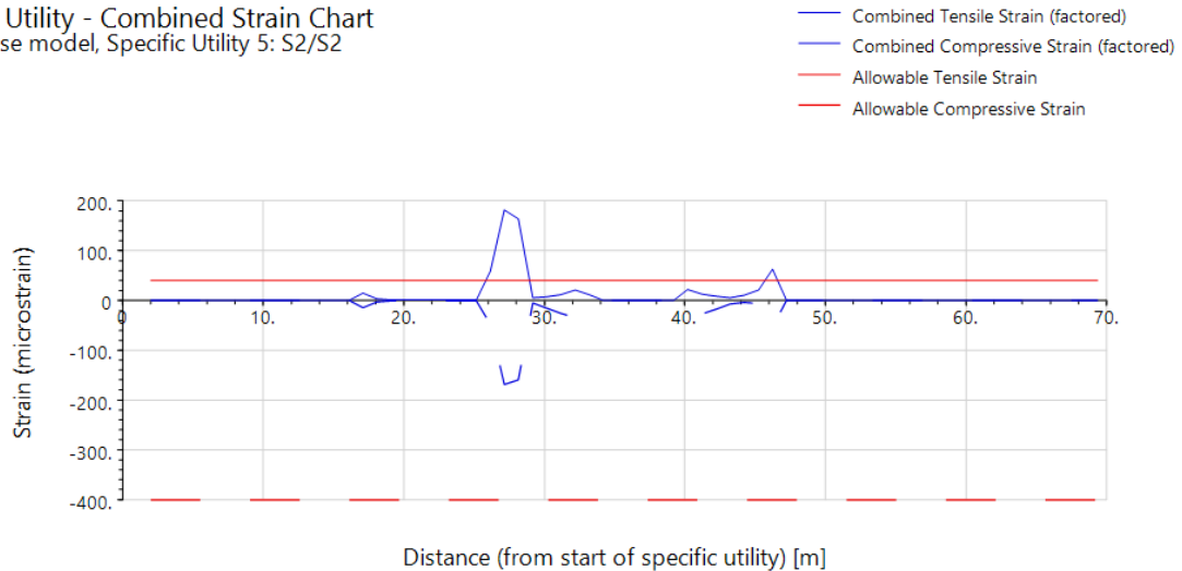
Figure 16.17: Combined strain profile of Sewer S2 – Method 2 CIRIA Excavation and Installation - based on smoothed deflection profile
