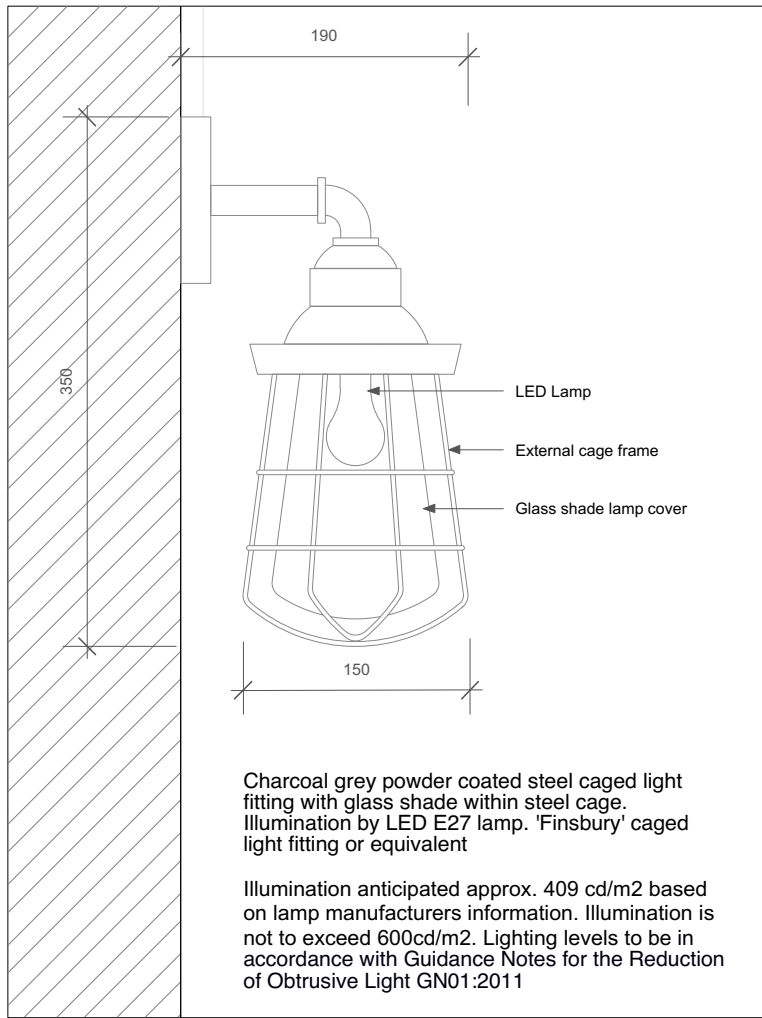
4 Wall Light Detail 1:5
