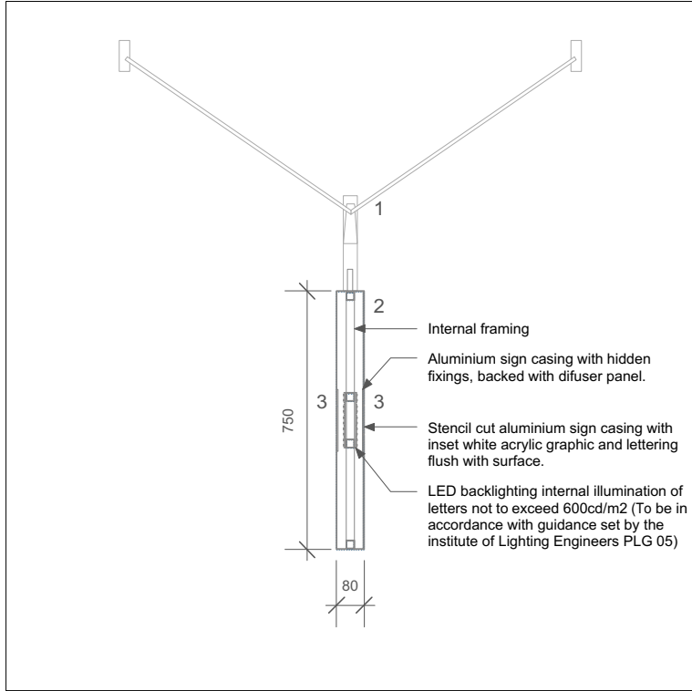
5 Signage Section Detail 1:20
