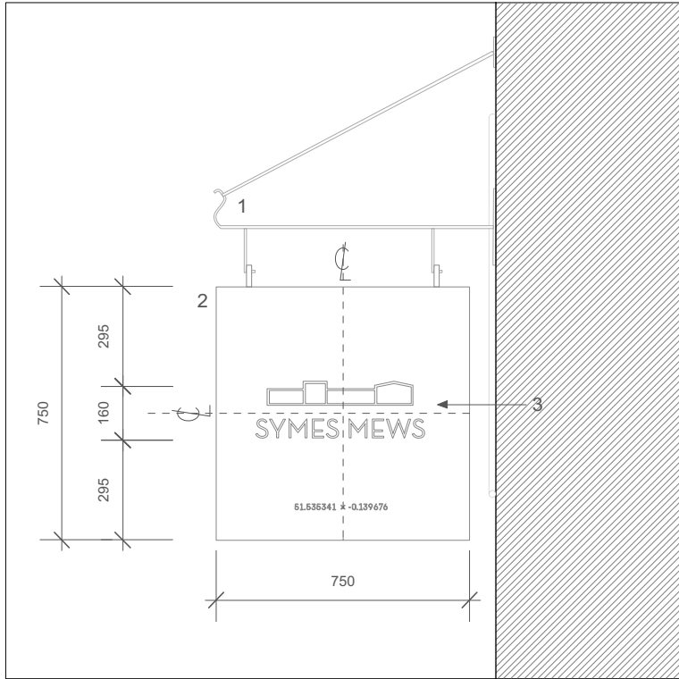
3 Signage Front Detail 1:20
