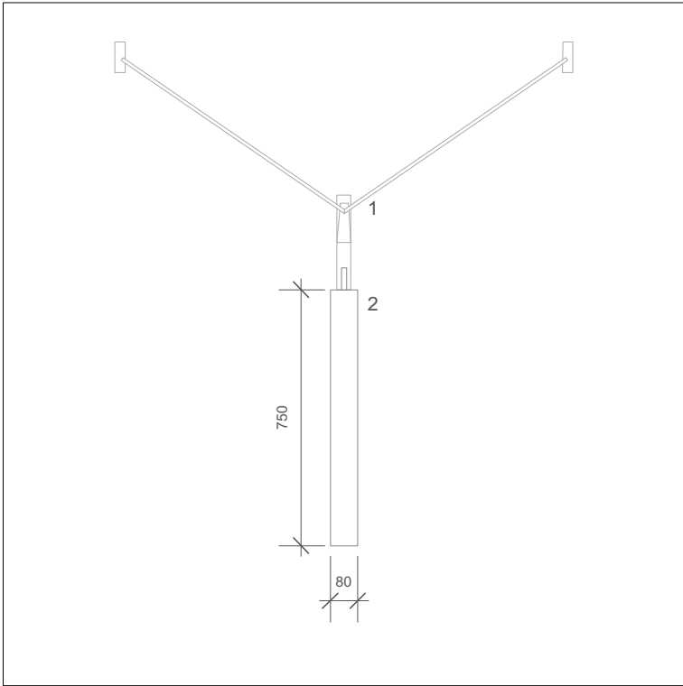
2 Signage Side Detail 1:20
