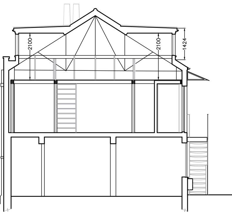
Section C - C
