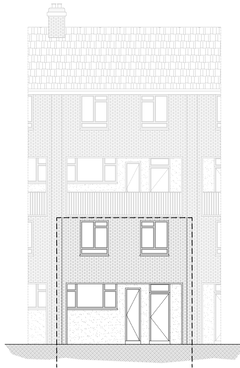
PROPOSED FRONT ELEVATION (not changes)
