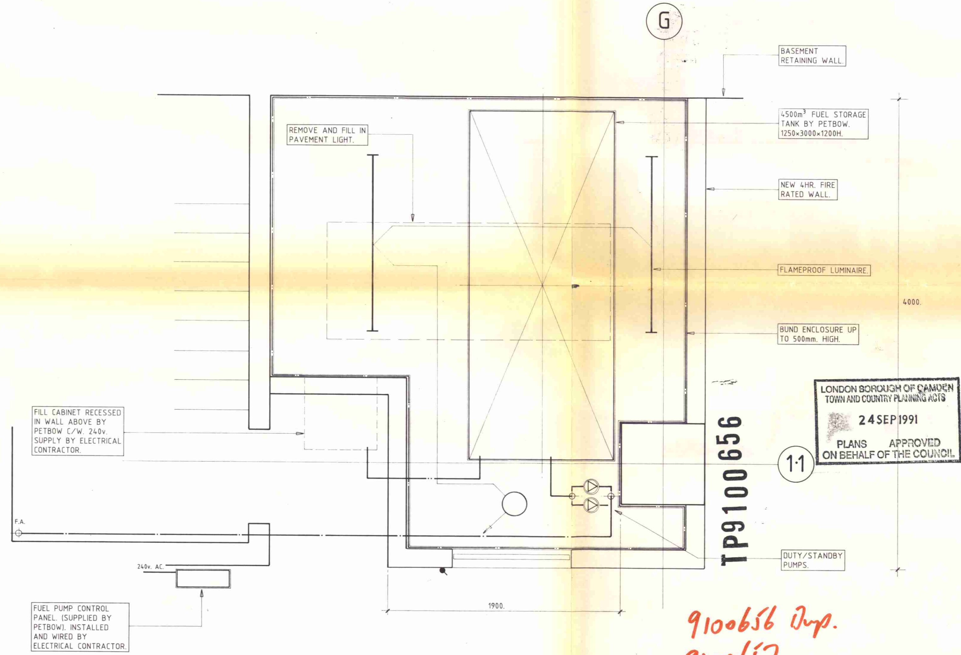
GENERATOR FUEL TANK ROOM, BASEMENT 1:20
