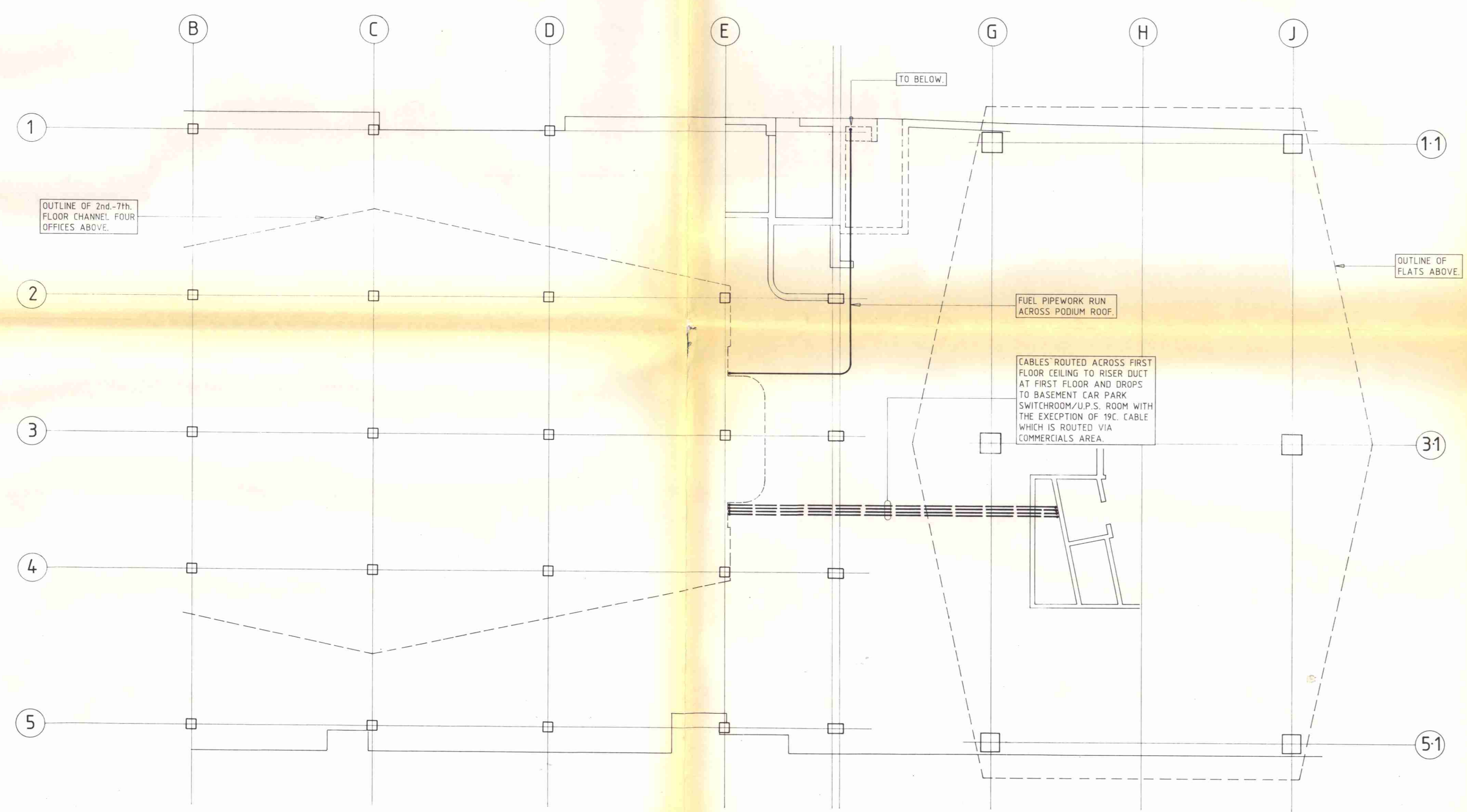
CABLE ROUTING PLAN, FIRST FLOOR 1:100
