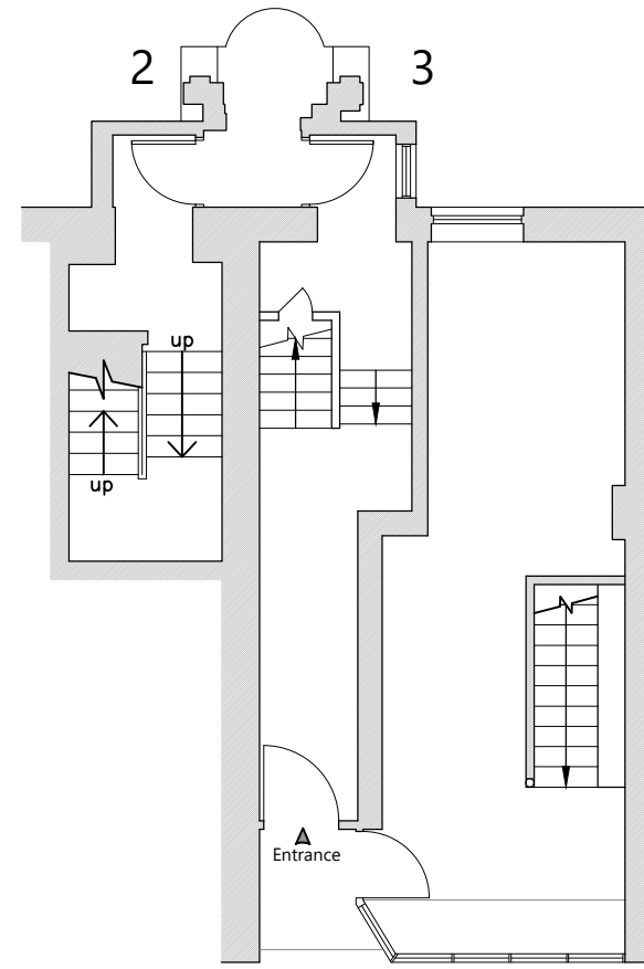
53 55 Ground Floor Plan As Existing
