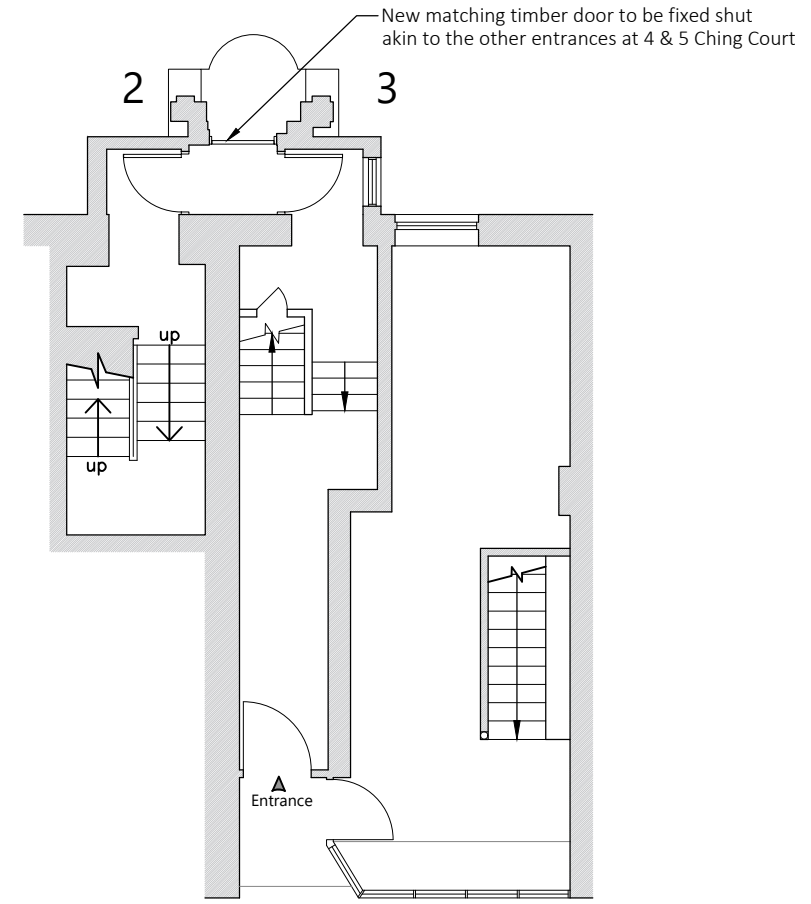
53 55 Ground Floor Plan As Proposed
