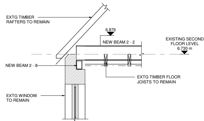
PROPOSED SECTION / ELEVATION 42
