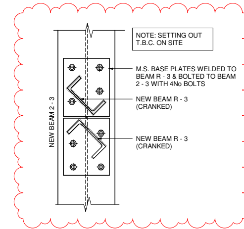
PROPOSED STEEL CONNECTION DETAIL E
