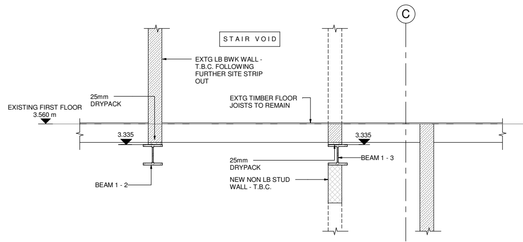
PROPOSED SECTION 40
