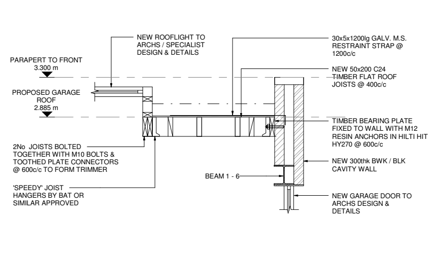
PROPOSED SECTION 41
