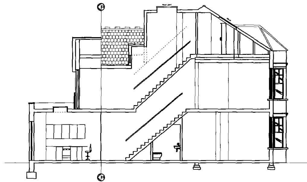
Proposed cross section D-D 1:100
