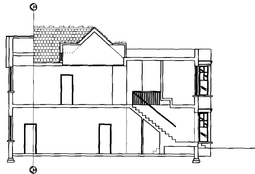
Existing cross section D-D 1:100
