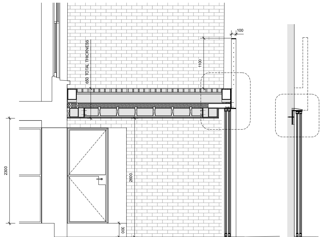
SECTION A
