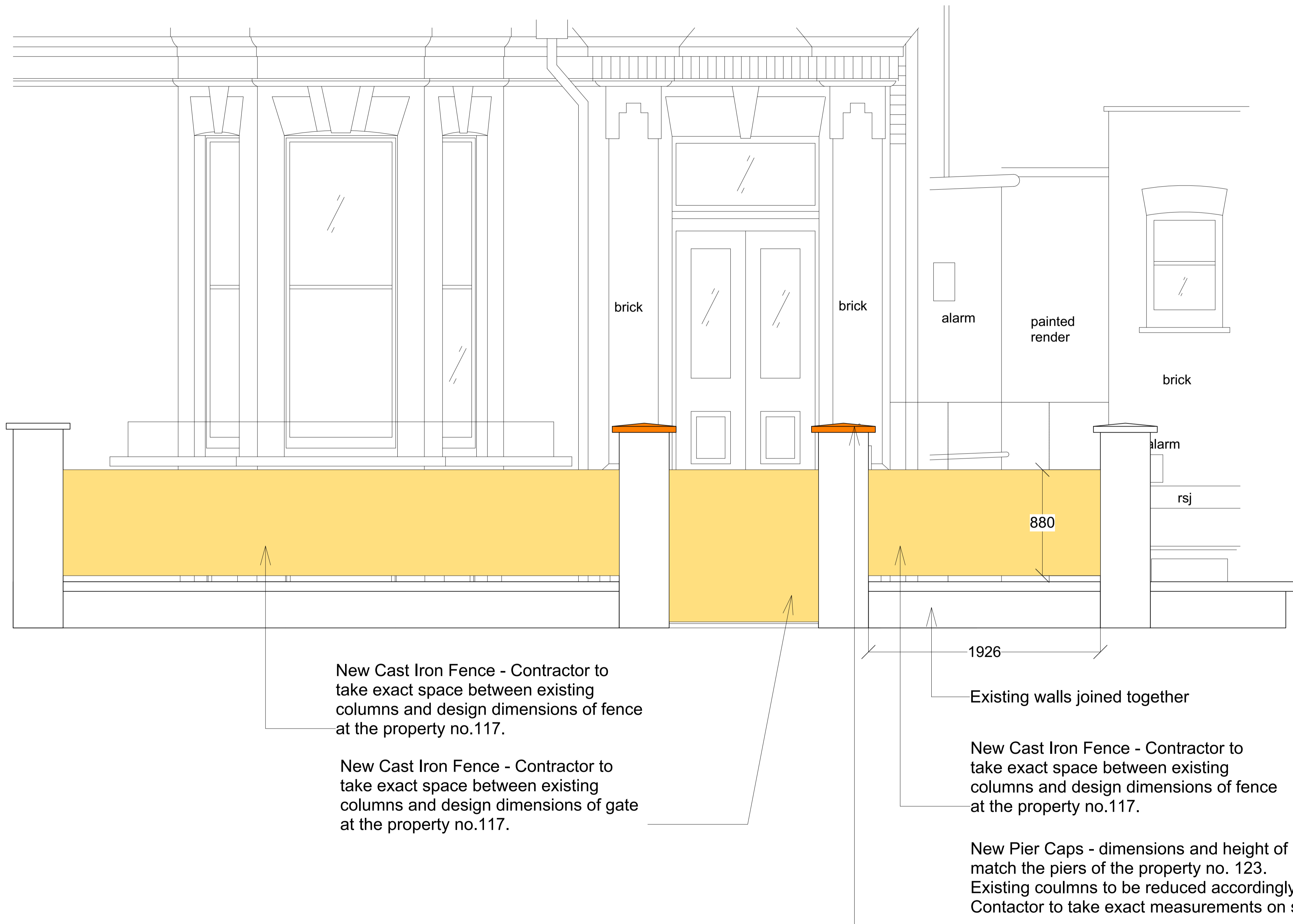
REFERENCE IMAGE: NEW PIER CAPS - DESIGN INTENT
