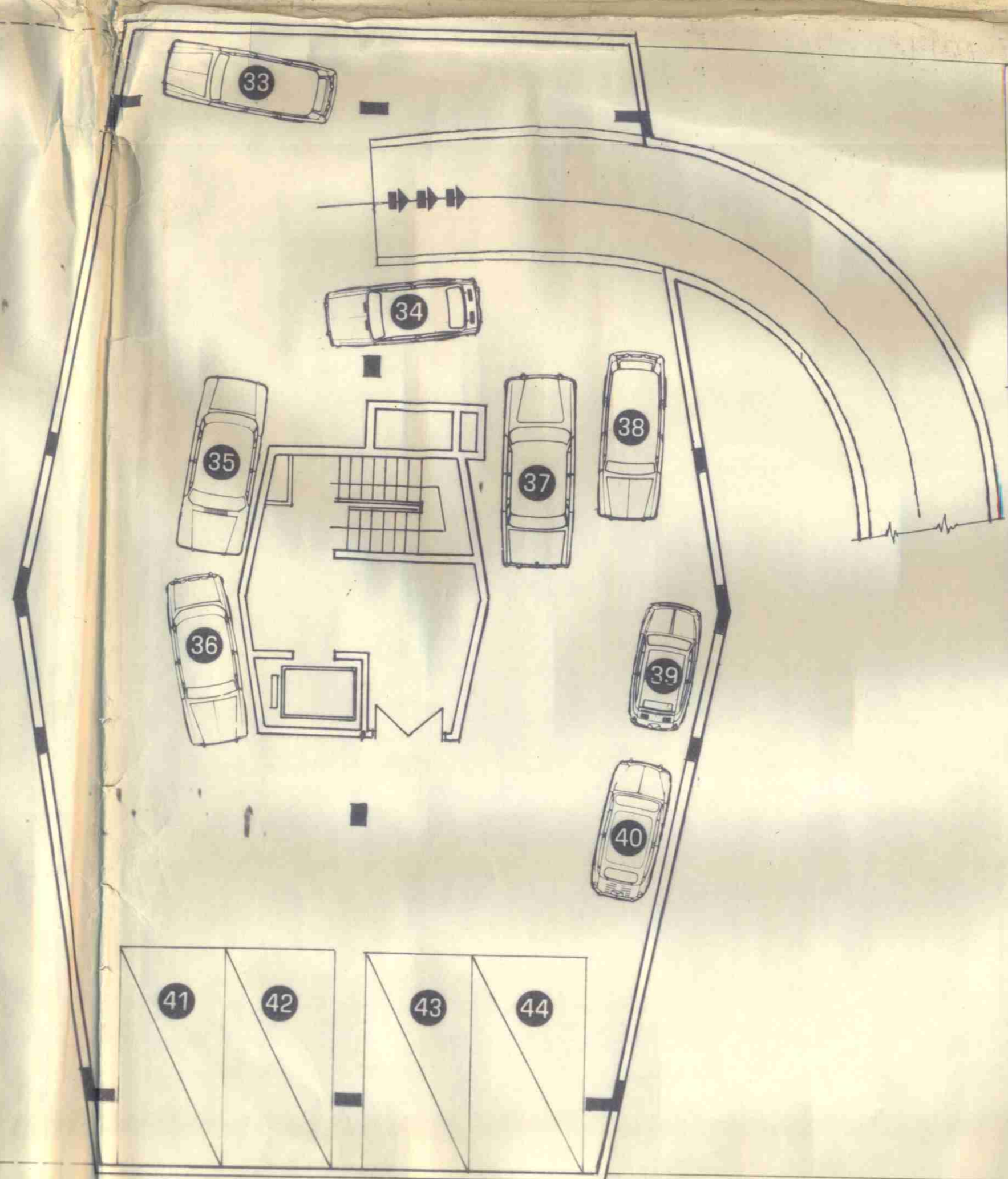
SUB-BASEMENT PLAN
