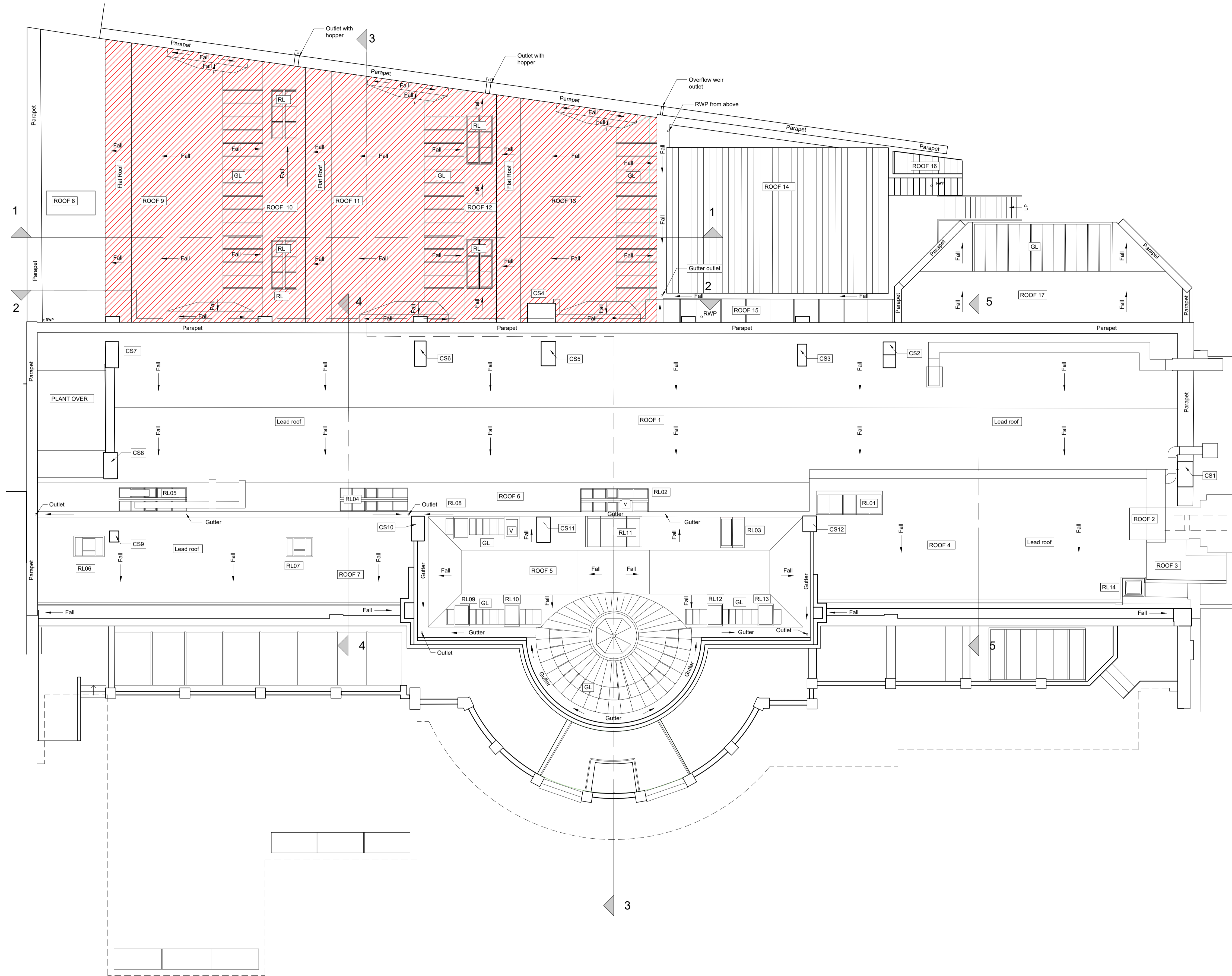
Roof Plan As Existing (Showing Demolition / Stripping Out)
