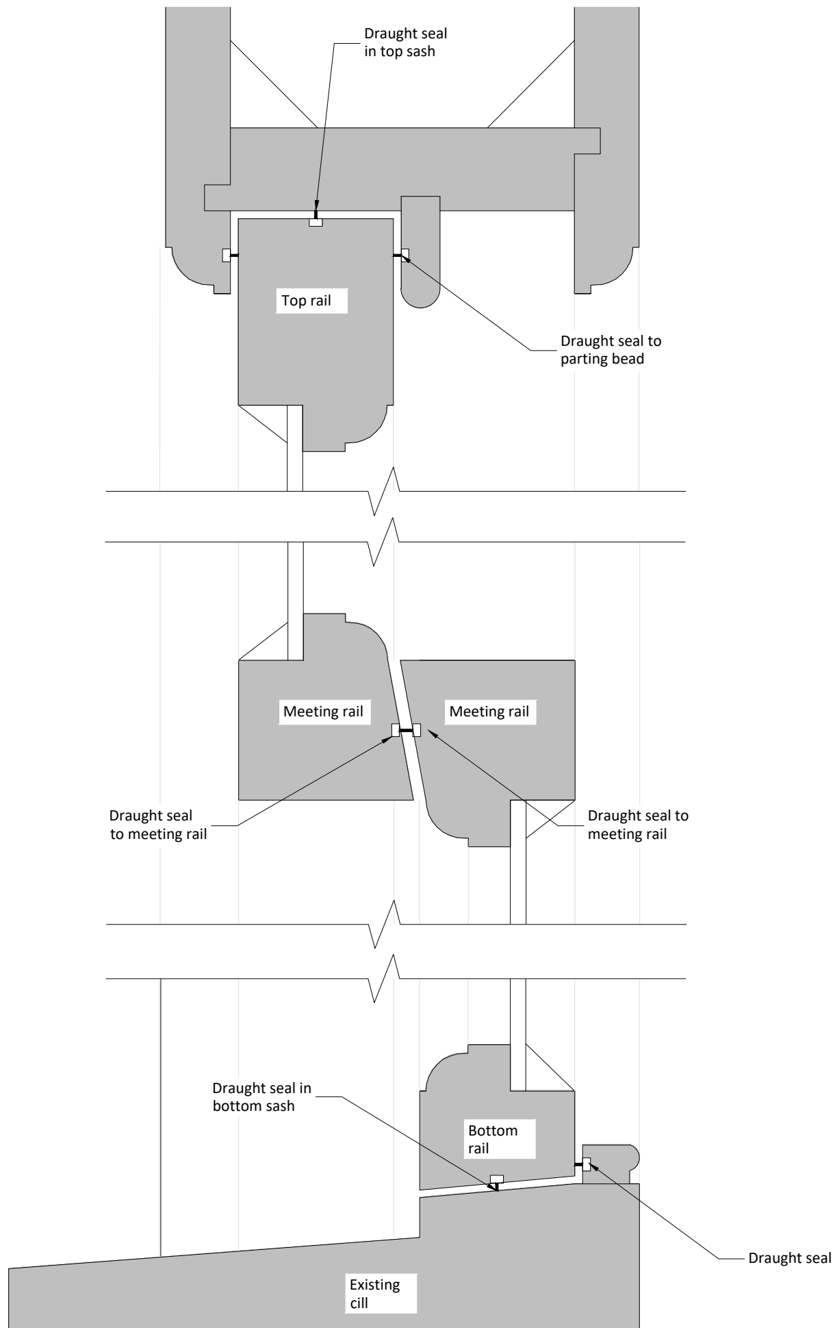
Typical Section Details Box Sash Window Draught Proofing
