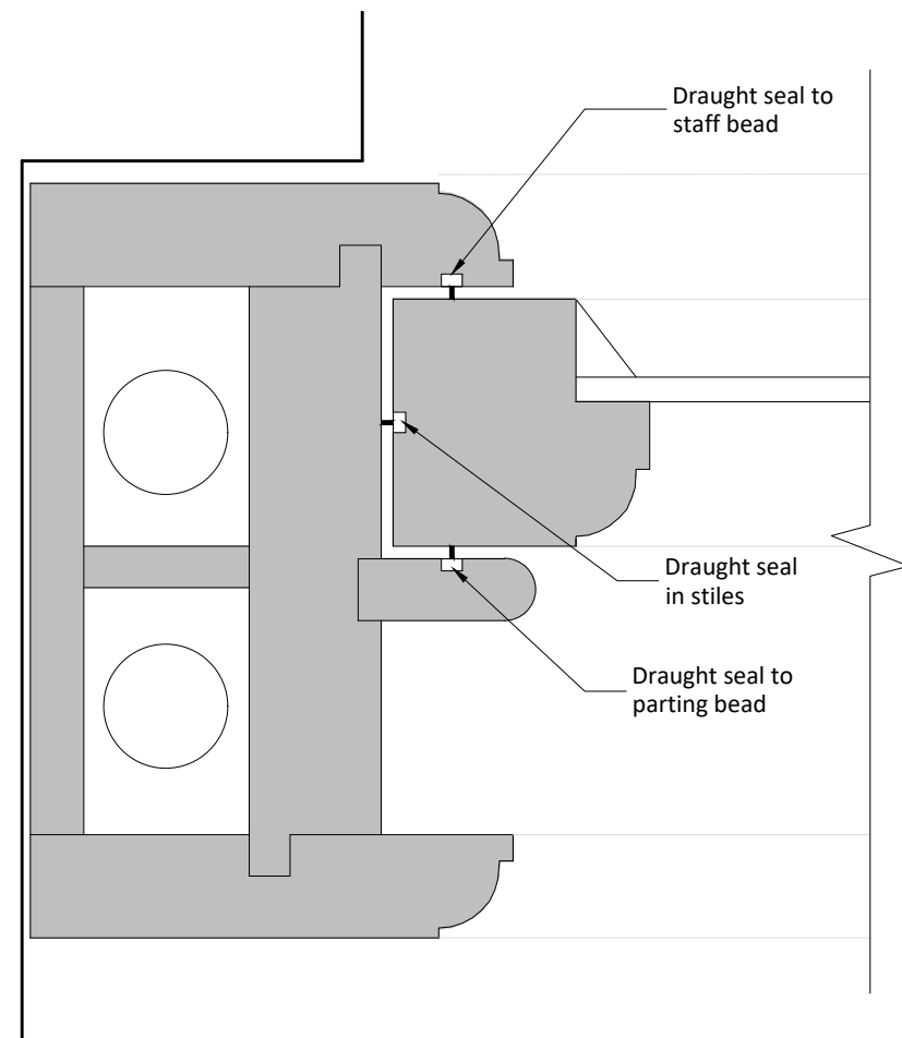
Typical Jamb Detail Box Sash Window Draught Proofing
