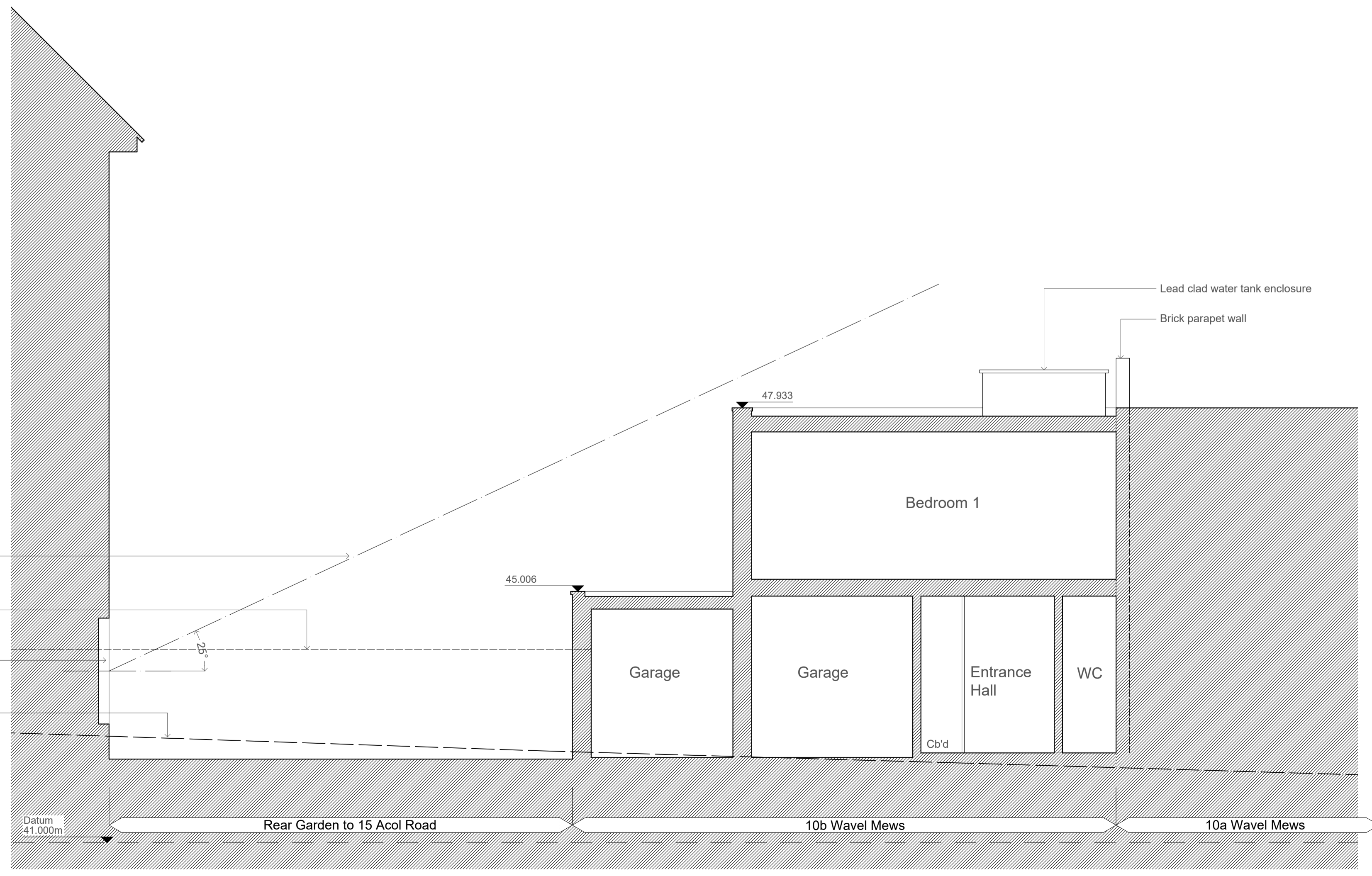
836/38 Existing Section AA 01 1:50 @ A1
