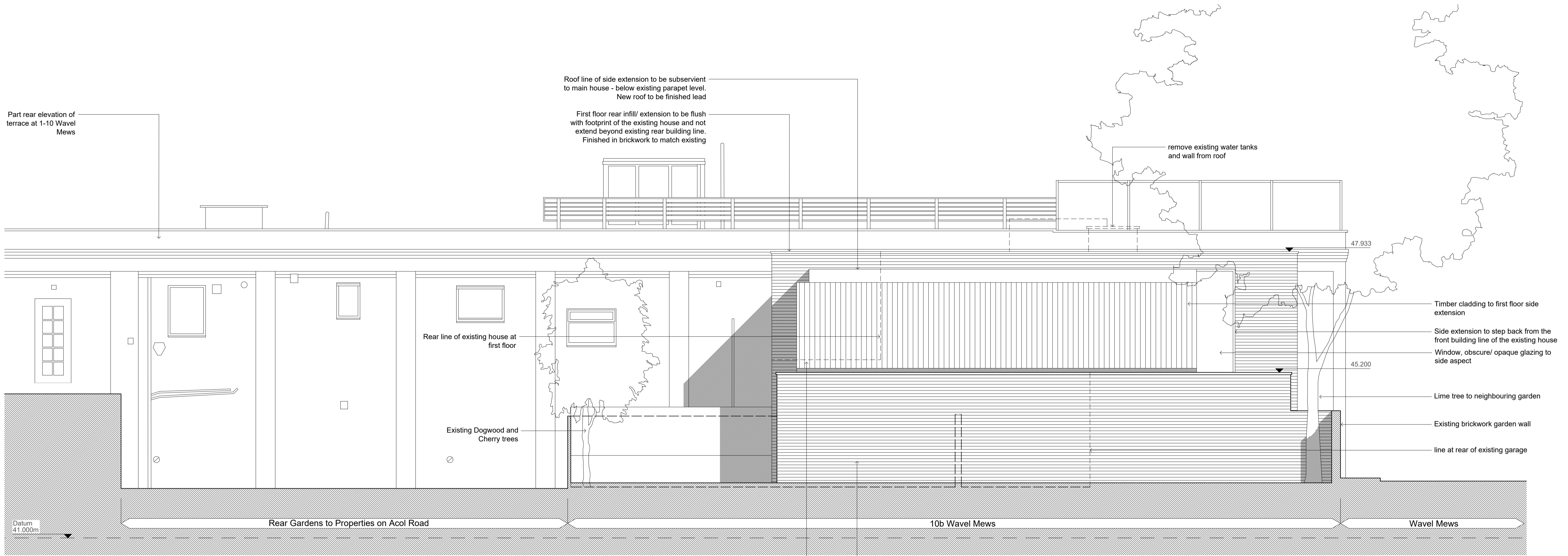
836/36 Proposed Side Elevation 02 1:50 @ A1
