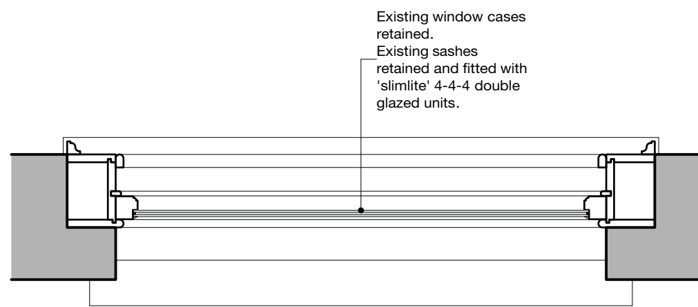
2 Proposed Window
