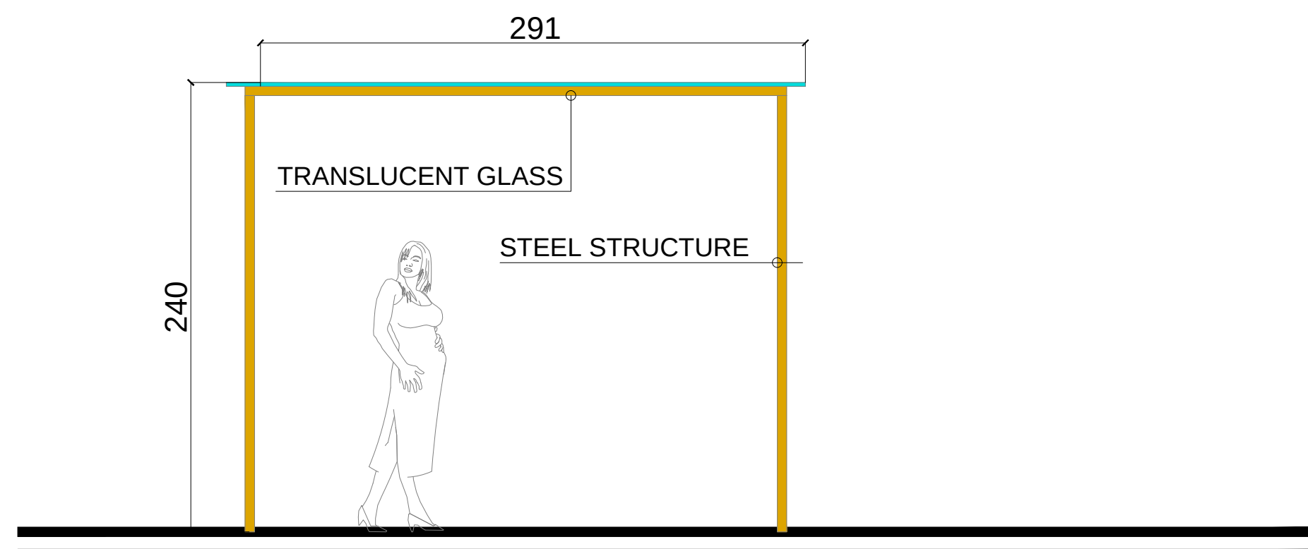
FRONT VIEW
