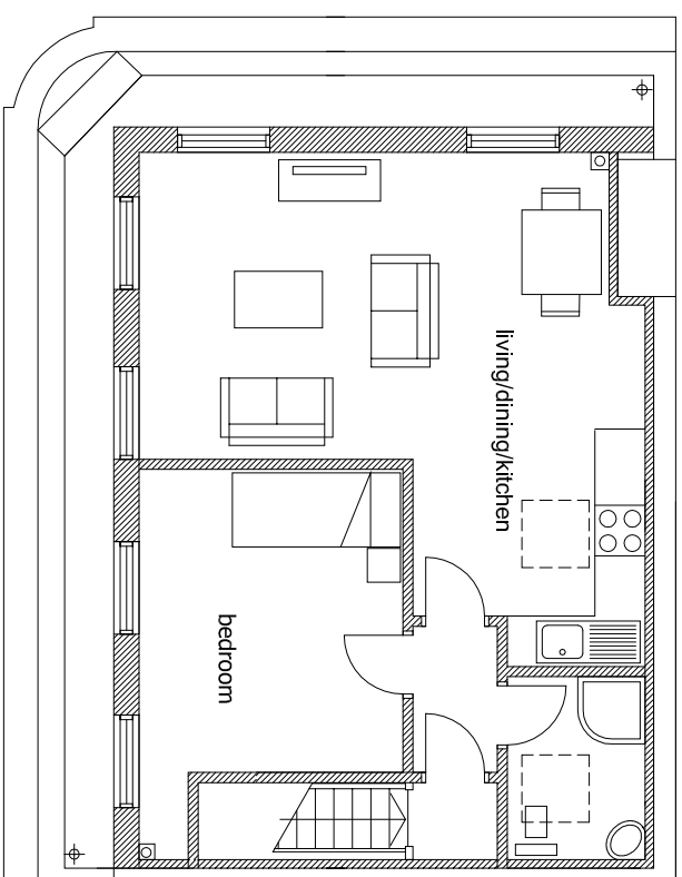
NEW FOURTH FLOOR AS PROPOSED 1B/1P FLAT GIA 46 M 2
