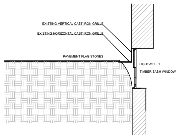
EXISTING SECTION DETAIL A-A @ 1:100
