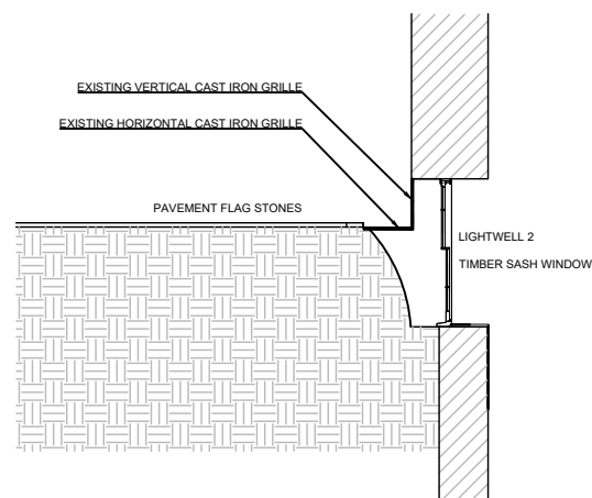
EXISTING SECTION DETAIL B-B @ 1:100
