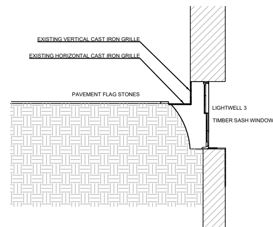
EXISTING SECTION DETAIL C-C @ 1:100
