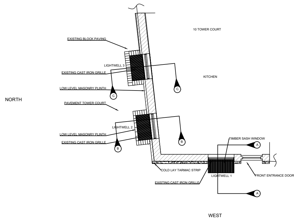
EXISTING FLOOR PLAN @ 1:100
