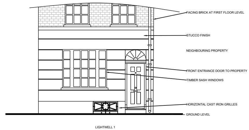
EXISTING WEST ELEVATION @ 1:100
