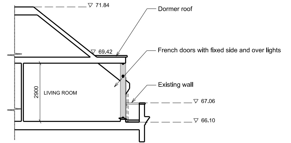
02 EXISTING SECTION A-A
