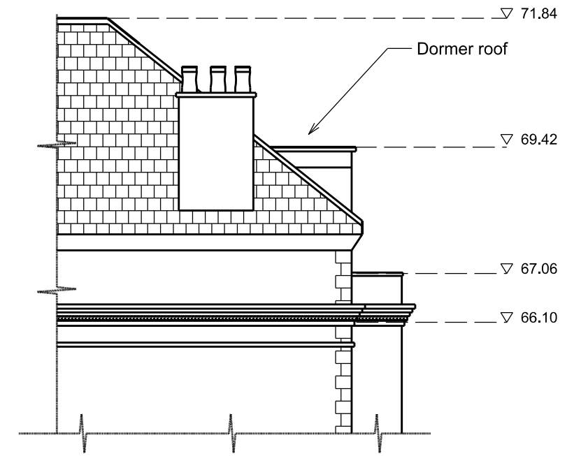
04 EXISTING SIDE ELEVATION
