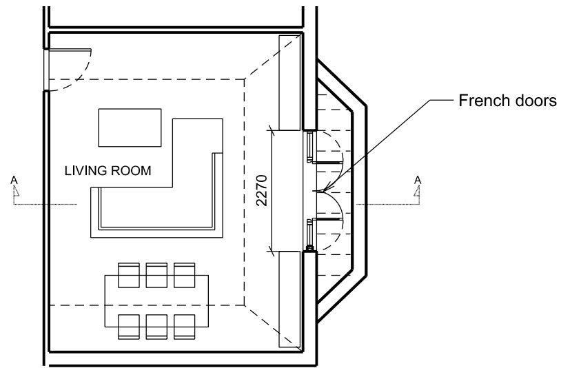
01 EXISTING PLAN
