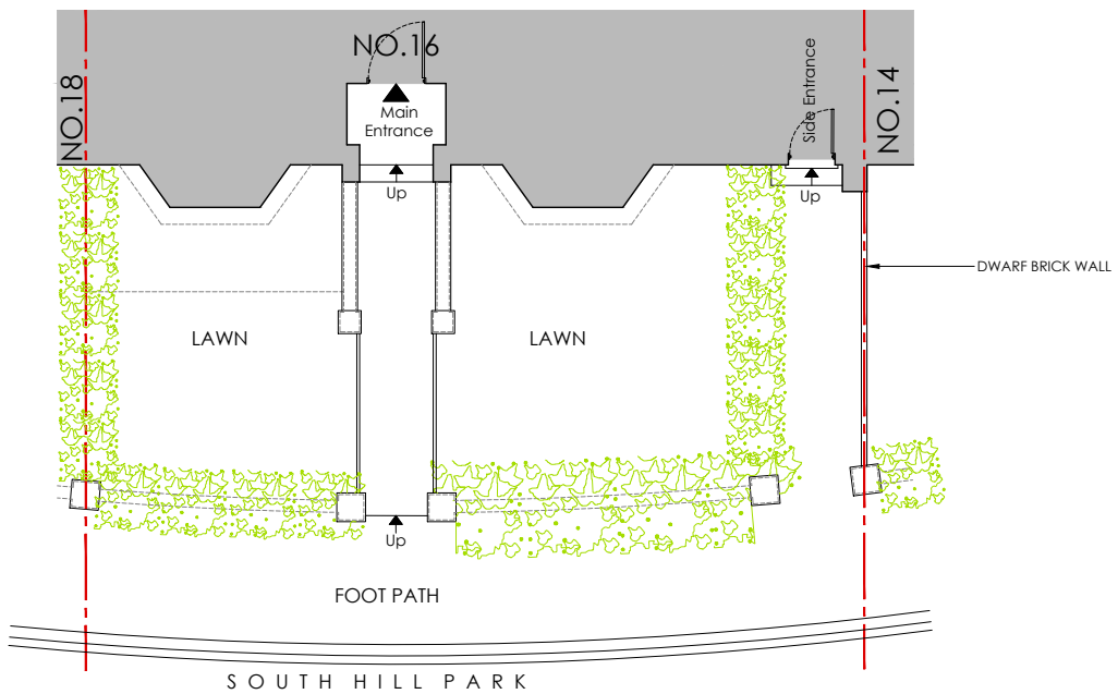
1 PLAN EXISTING 1:100
