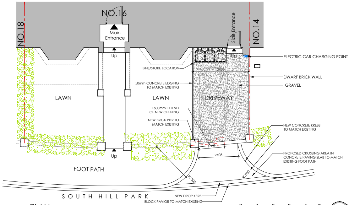
2 PLAN PROPOSED 1:100
