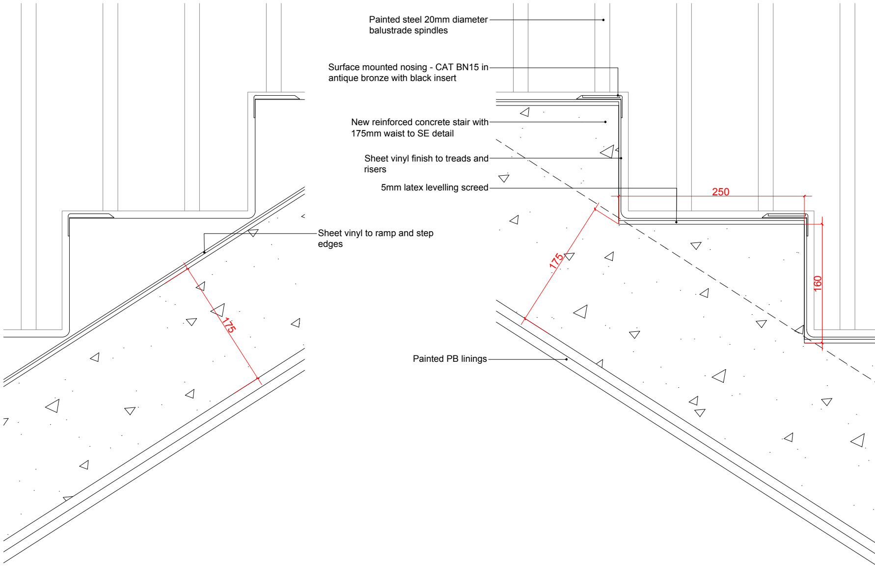
00 A5122 Detailed Section: Cycle Channel Stair 02_1:5
