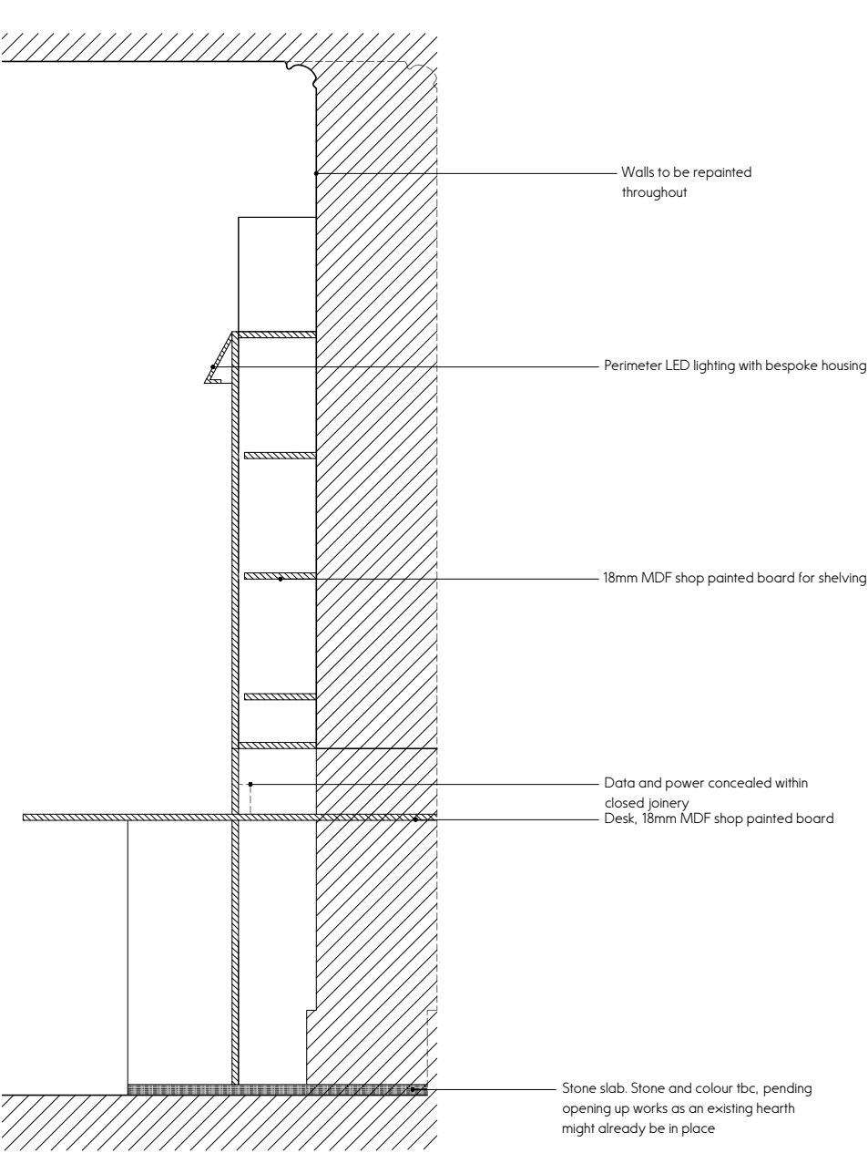
3 7.11 PROPOSED JOINERY SECTION CC SCALE 1:20 @ A3
