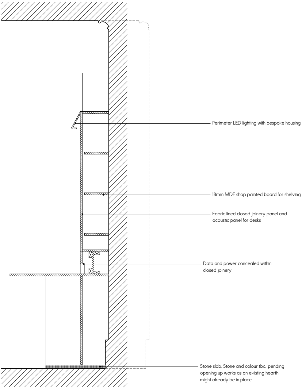
4 7.11 PROPOSED JOINERY SECTION DD SCALE 1:50 @ A3
