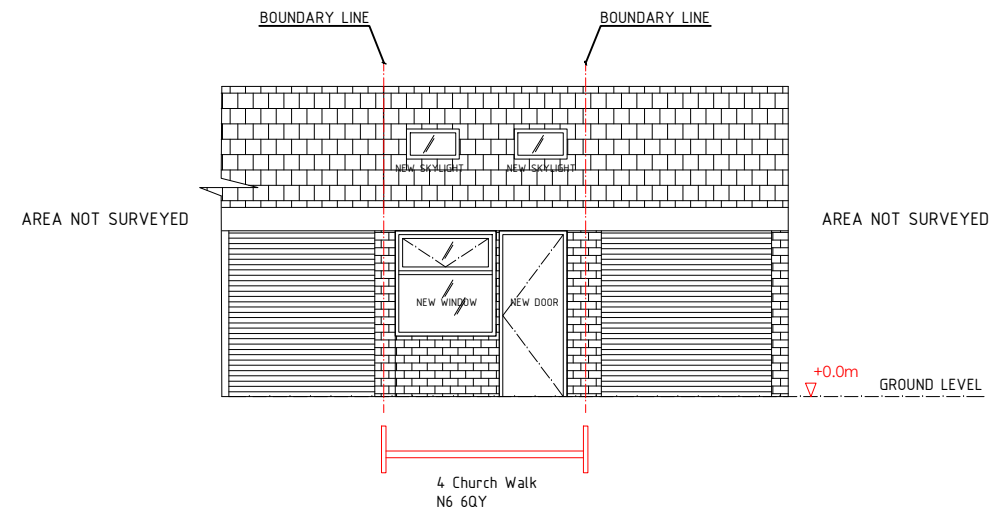
GARAGE-SOUTH-EAST-ELEVATION-AS-PROPOSED
