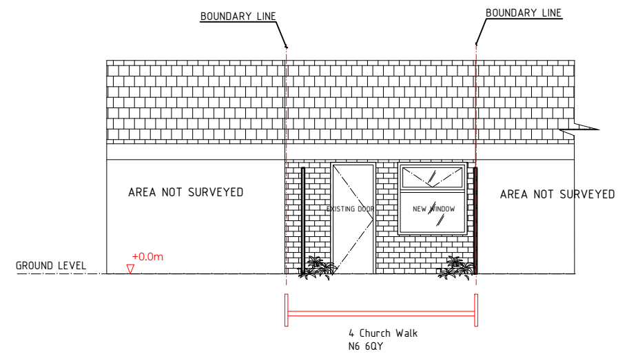
GARAGE-NORTH-WEST-ELEVATION-AS-PROPOSED
