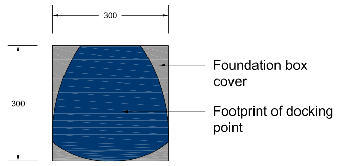
Docking Point and Foundation Box Cover - Plan View at Docking Point base
