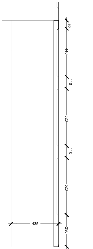
BILLIARDS ROOM PANELED DOOR SECTION SCALE 1:20
