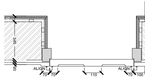
BILLIARDS ROOM PANELED DOOR PLAN SECTION SCALE 1:20
