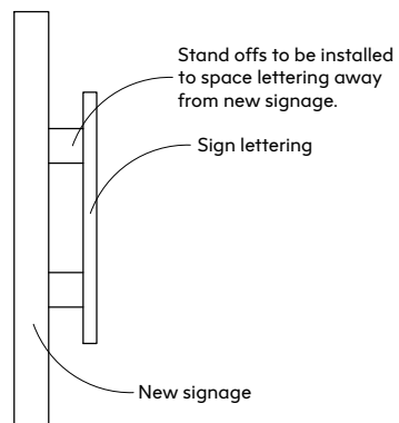
SIGNAGE SECTION (not to scale)
