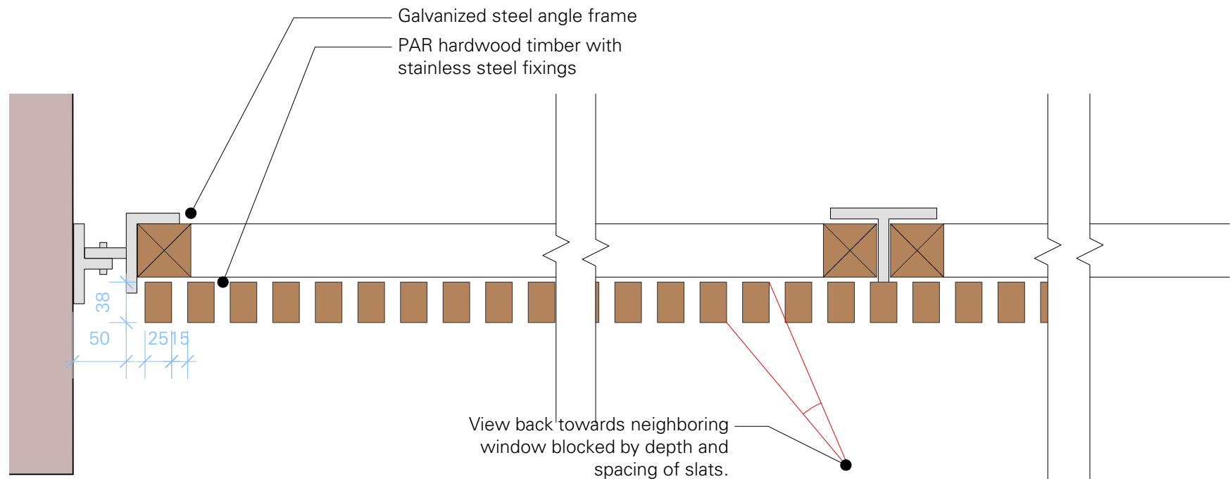
1 Vision Screen Plan Detail 317 Scale: 1:5
