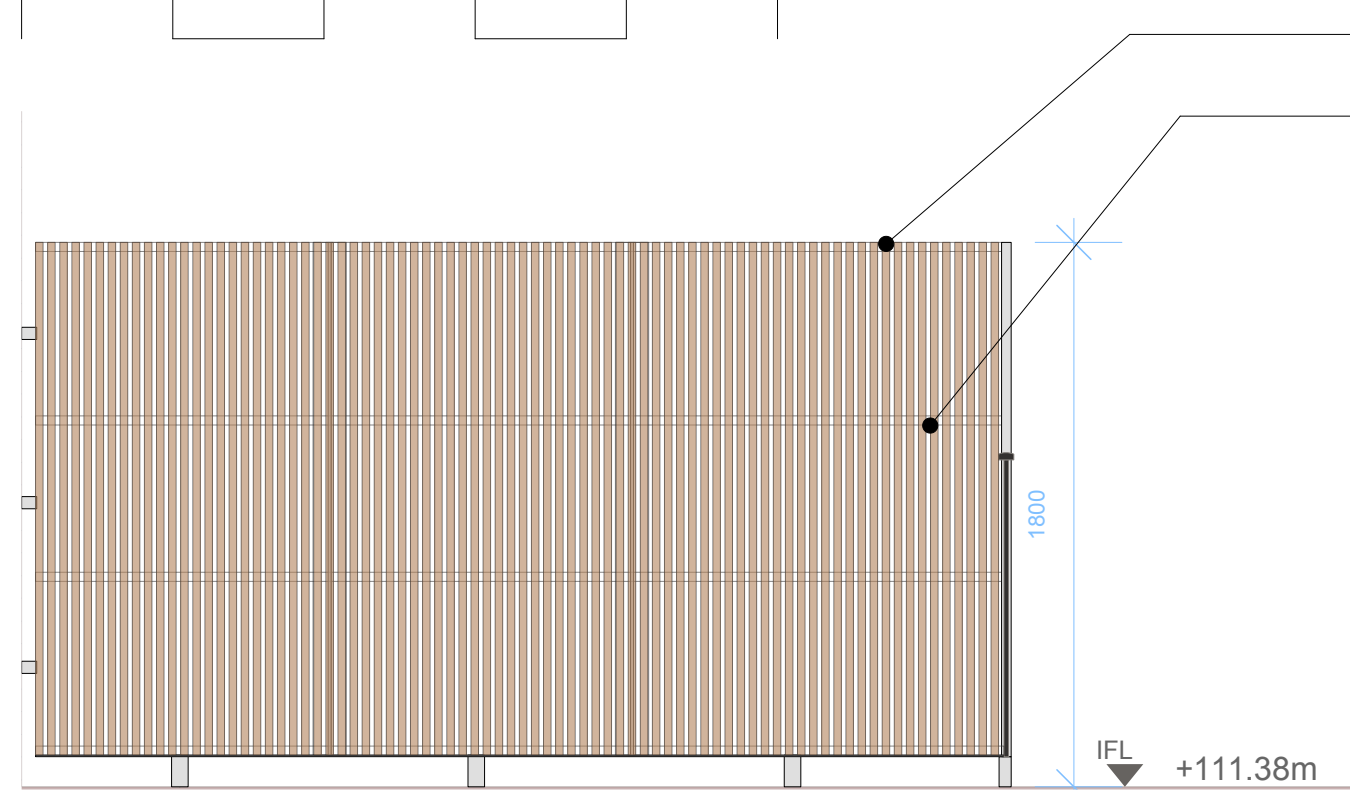
3 Vision Screen Elevation view towards Lakeview 317 Scale: 1:25
