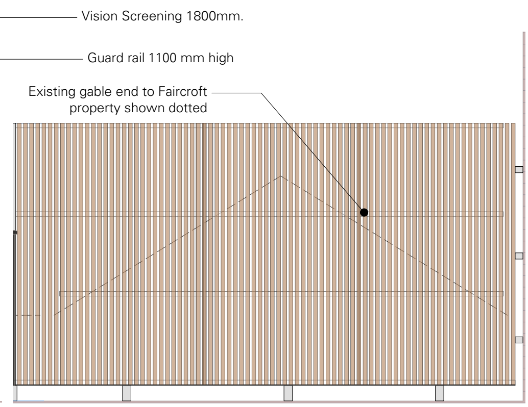
4 Vision Screen Elevation view towards Faircroft 317 Scale: 1:25
