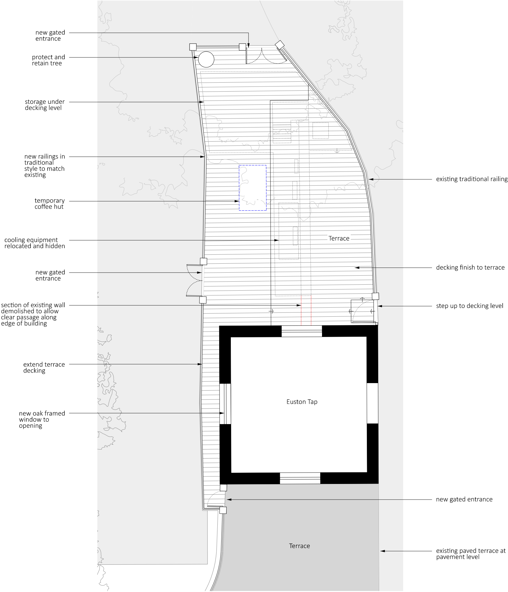
01 Proposed Ground Floor Plan
